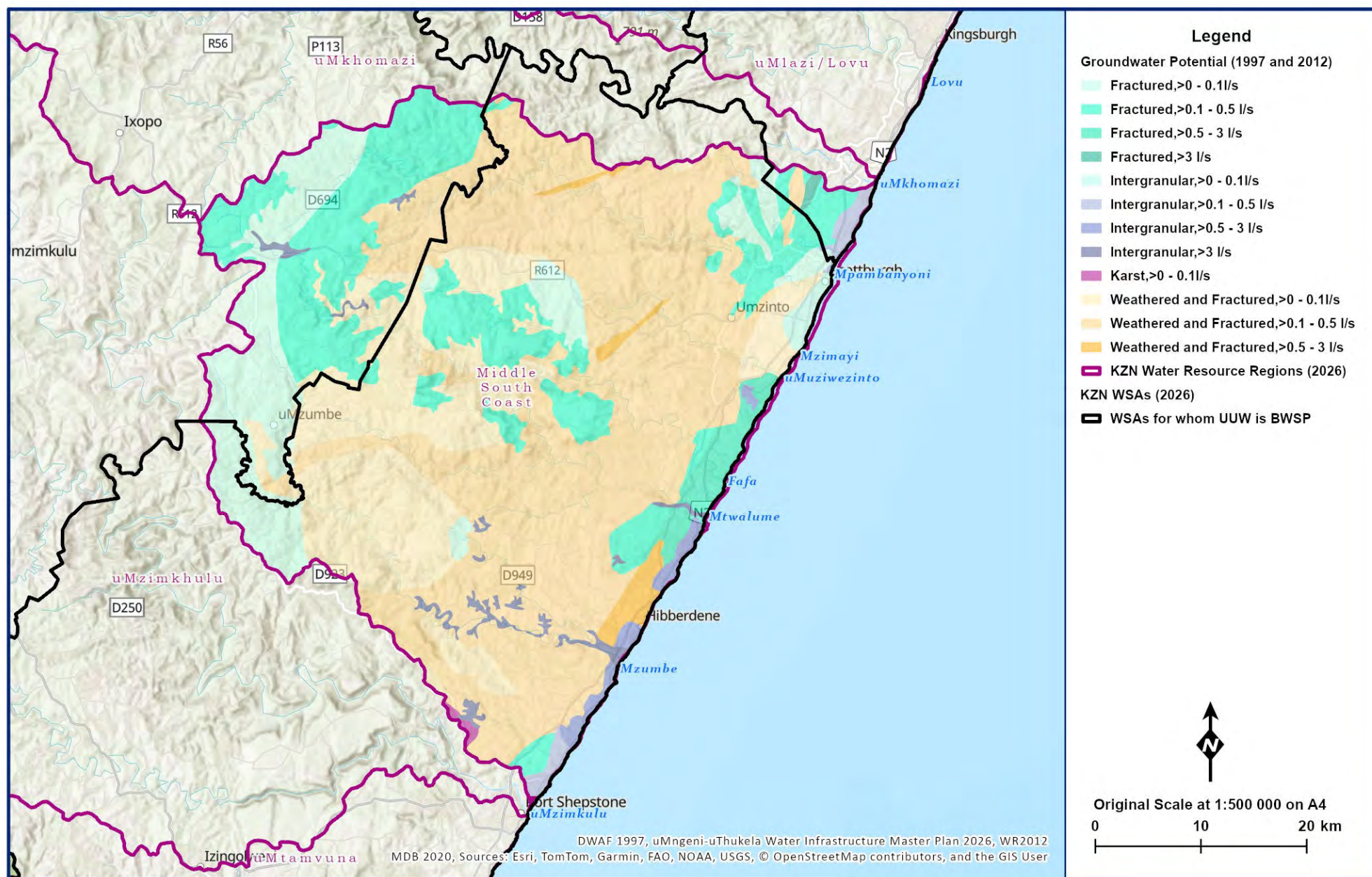
Figure 11.9 Groundwater potential in the Middle South Region.
