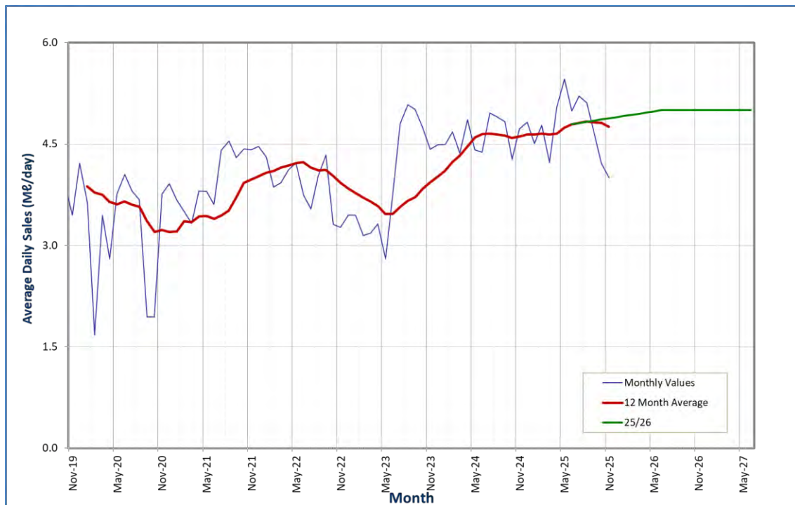
Figure 11.60 Water demand from Weza WTP.
