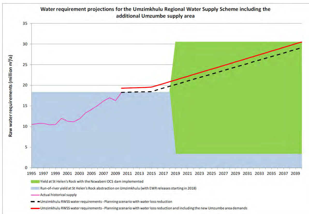
Figure 11.76 Water Balance Lower South Coast.
