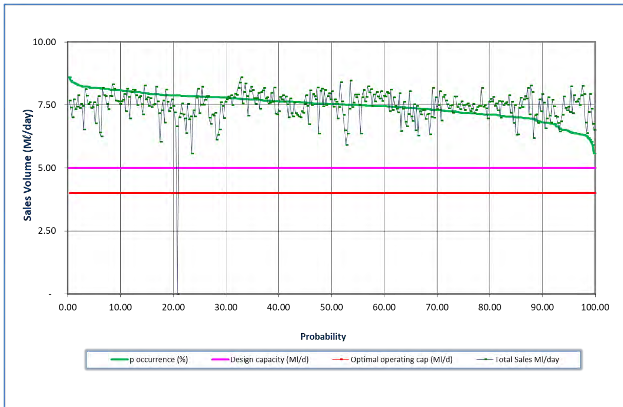
Figure 11.37 Analysis of historical production at Mhlabatshane WTP (December 2024 to November 2025).
