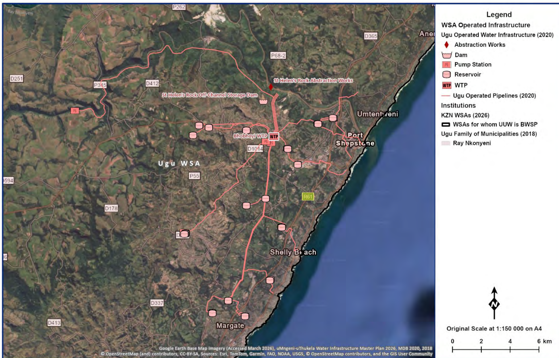
Figure 11.30 uMzimkhulu Supply System.
