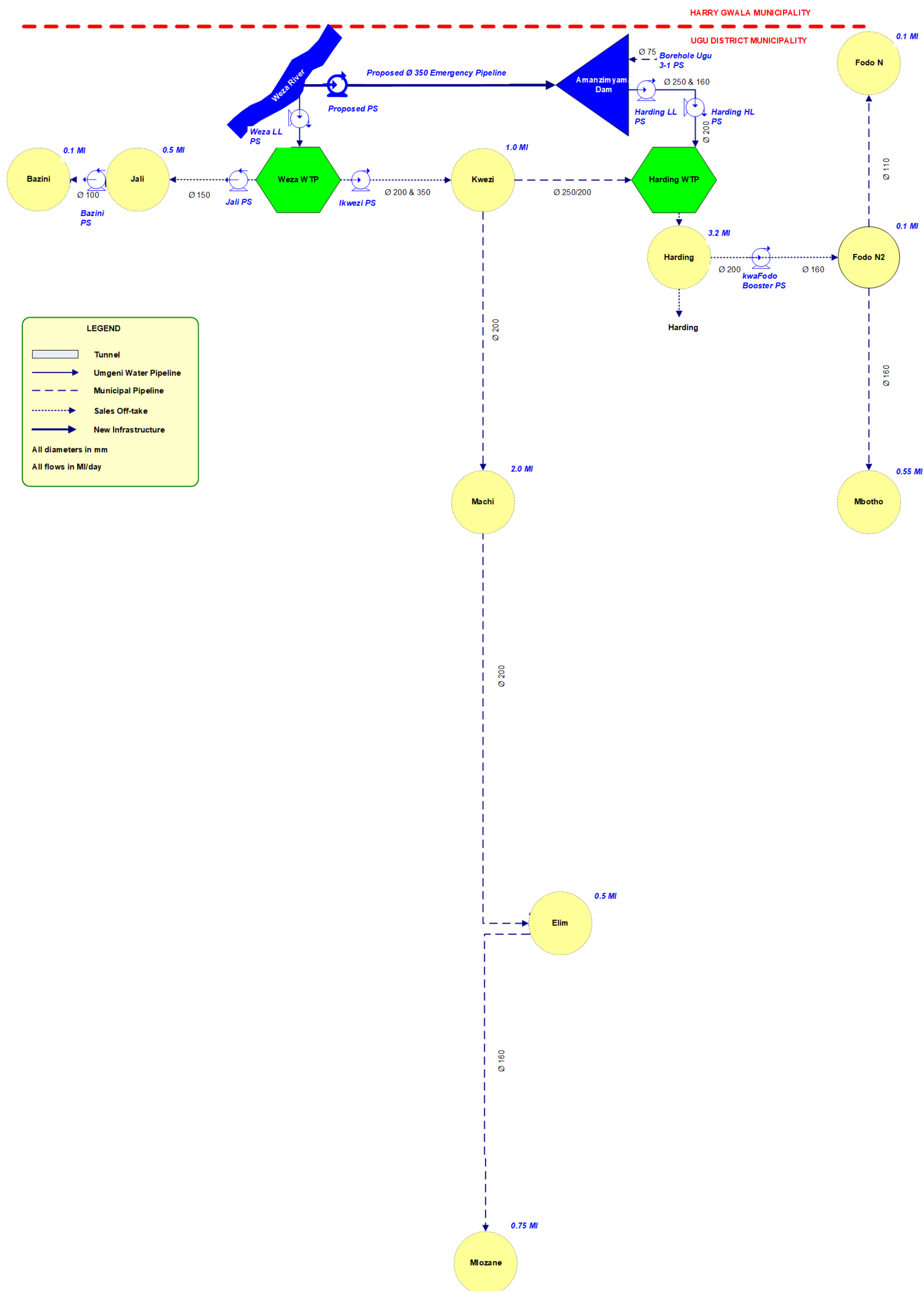
Figure 11.51 Schematic of the Harding-Weza System Bulk Supply Infrastructure.
