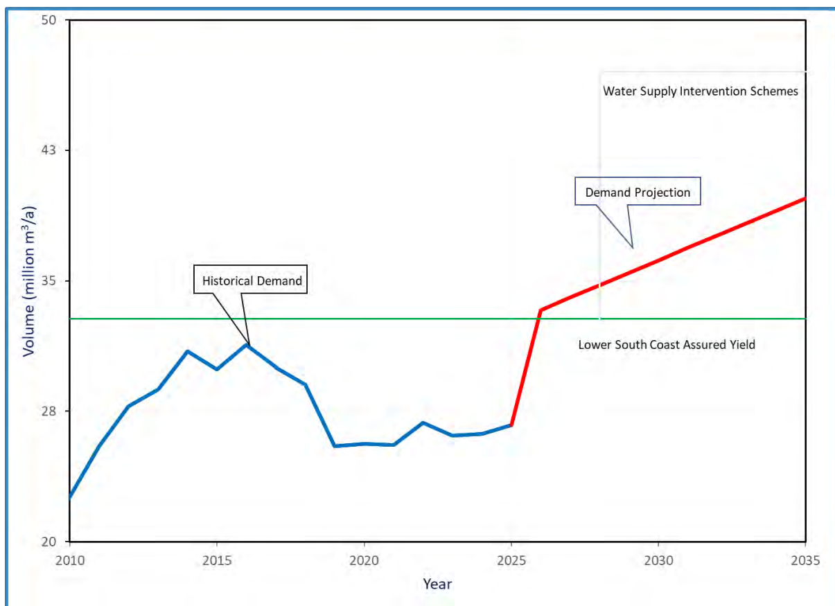
Figure 11.63 Lower South Coast water requirement projection scenarios.
