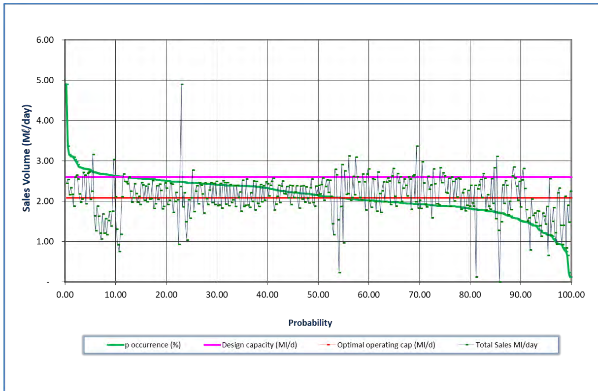
Figure 11.40 Analysis of historical production at Harding WTP (December 2024 to November 2025).
