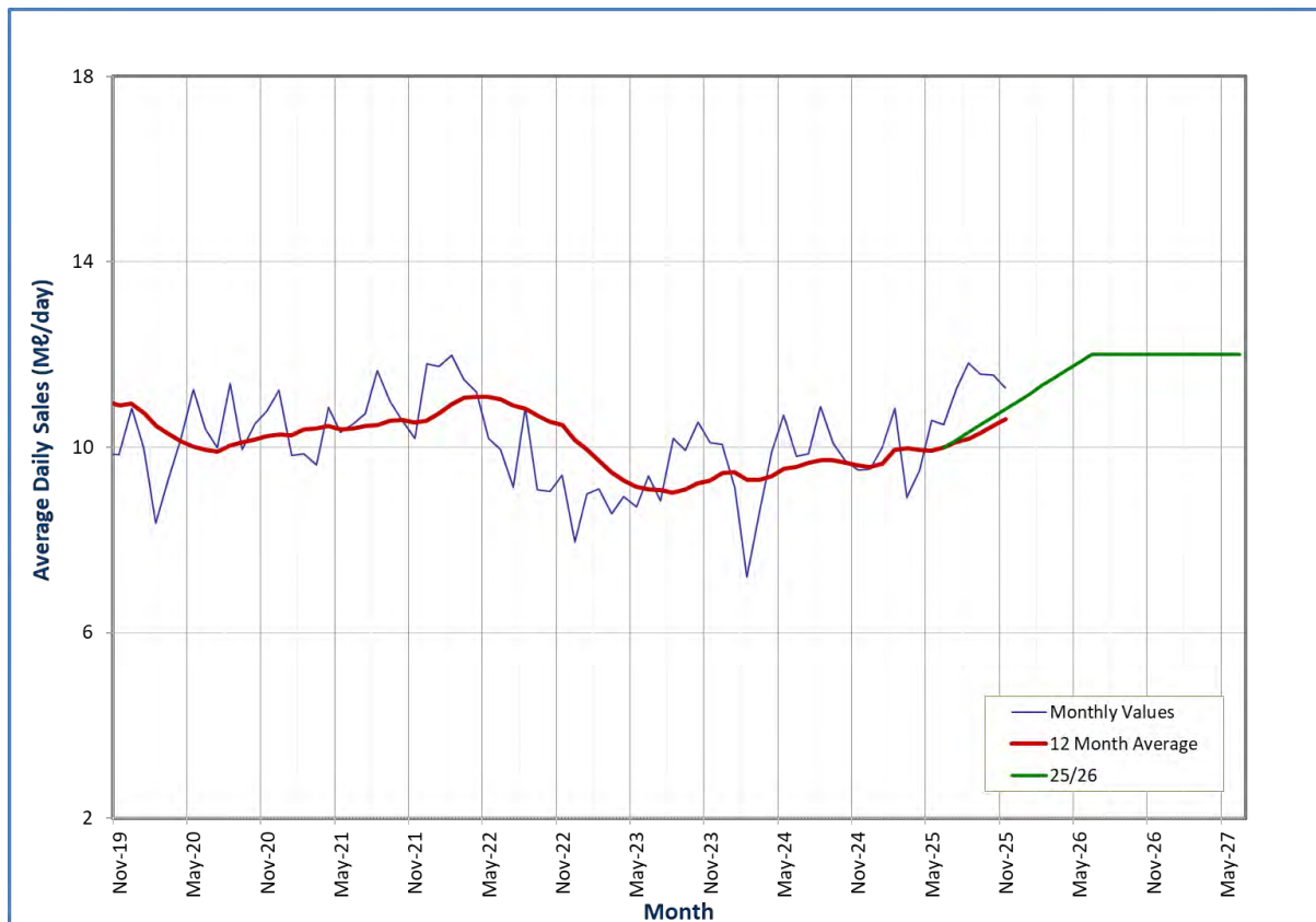
Figure 11.54 Water demand from Umzinto WTP.
