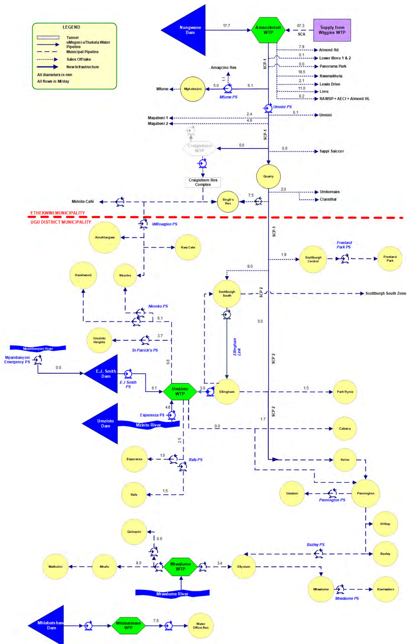
Figure 11.43 Demand on the South Coast System as at November 2025.
