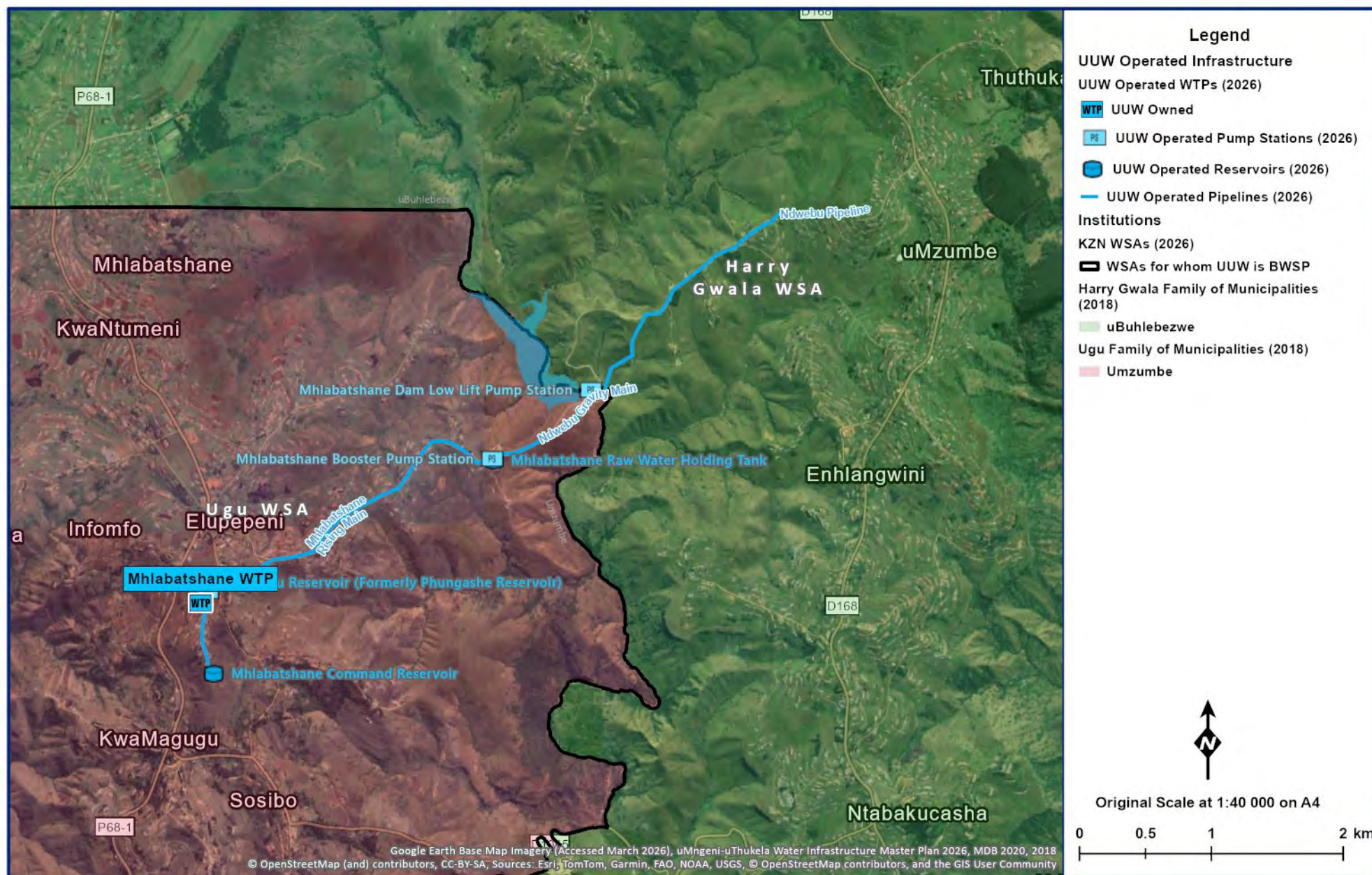
Figure 11.29 Mhlabatshane Supply System.
