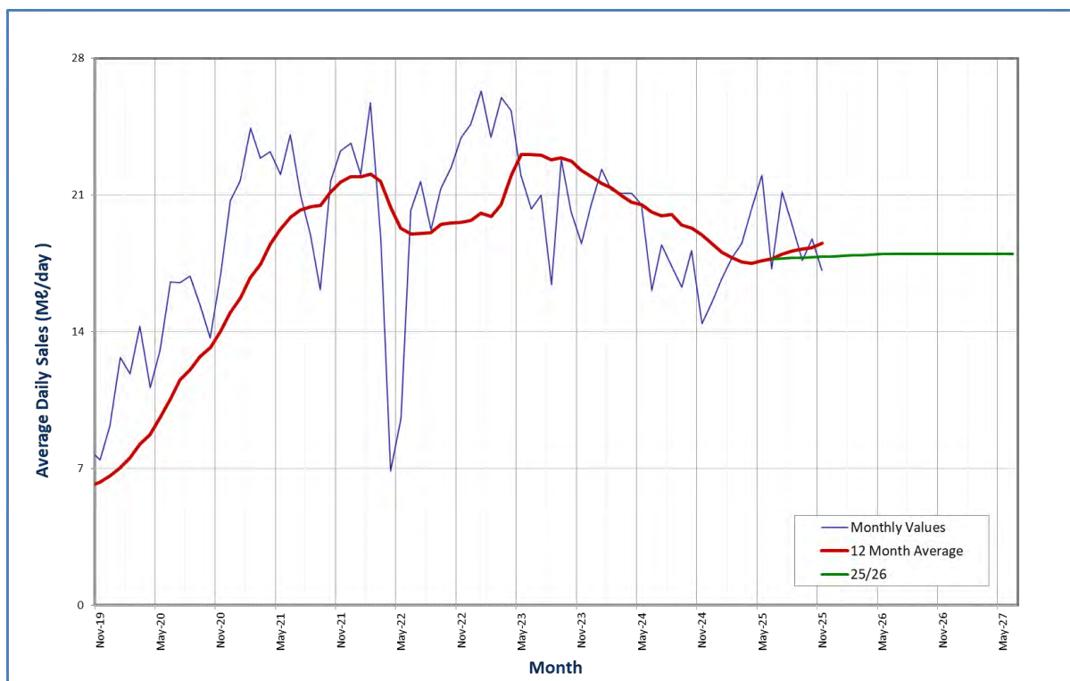
Figure 11.53 Water demand from Amanzimtoti WTP.
