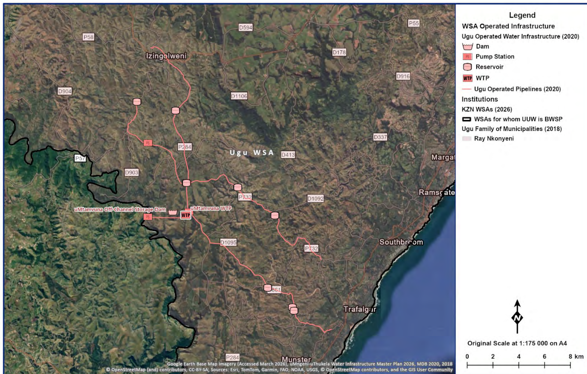
Figure 11.31 uMtavuna Supply System.
