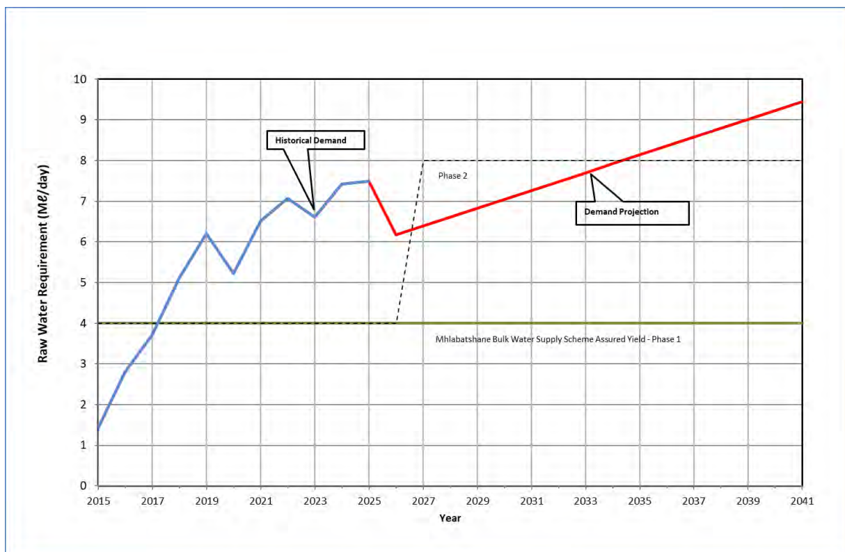
Figure 11.72 Water Balance Mhlabatshane BWSS.
