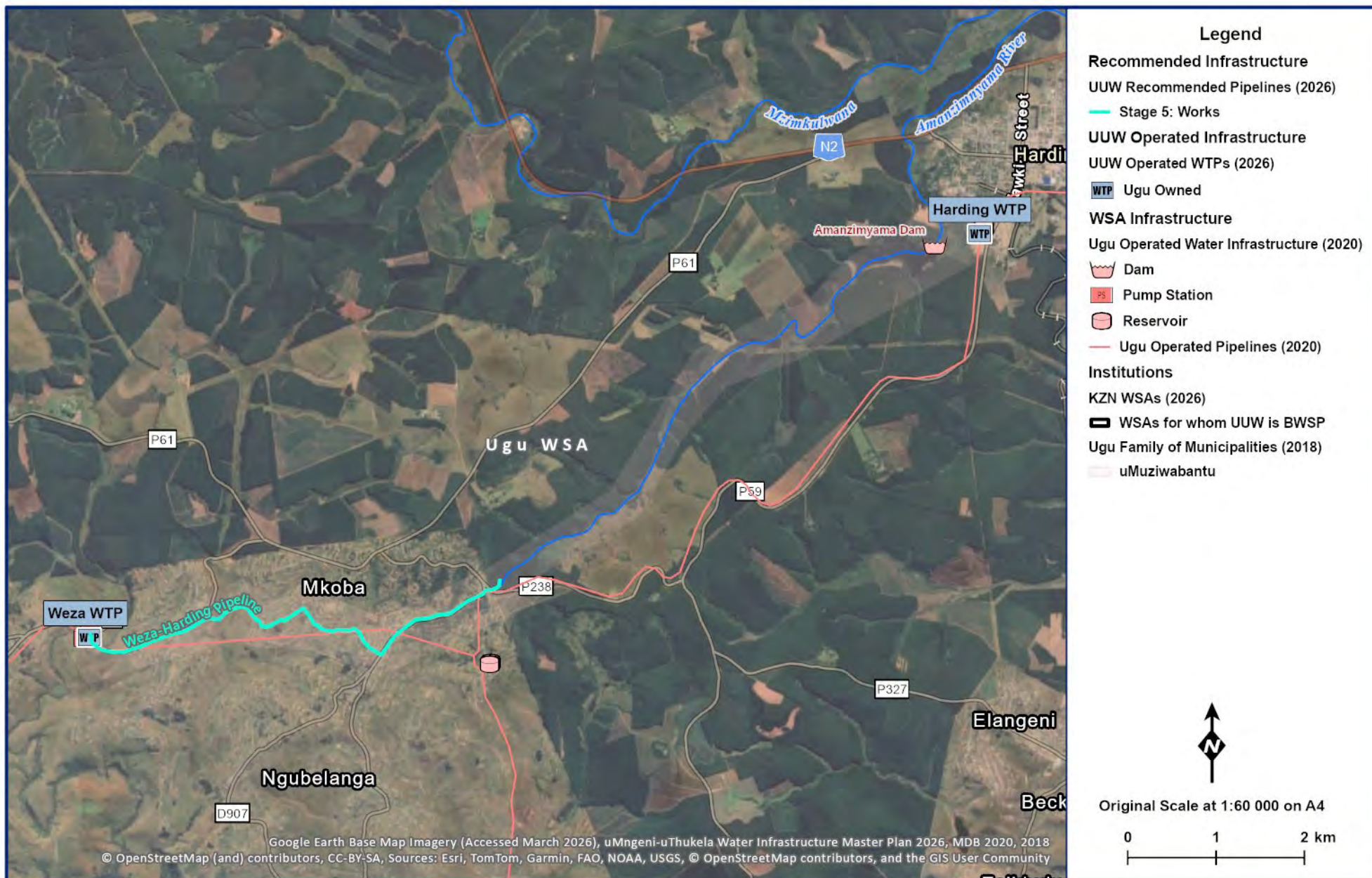
Figure 11.78 General layout of the Weza River Emergency Scheme.
