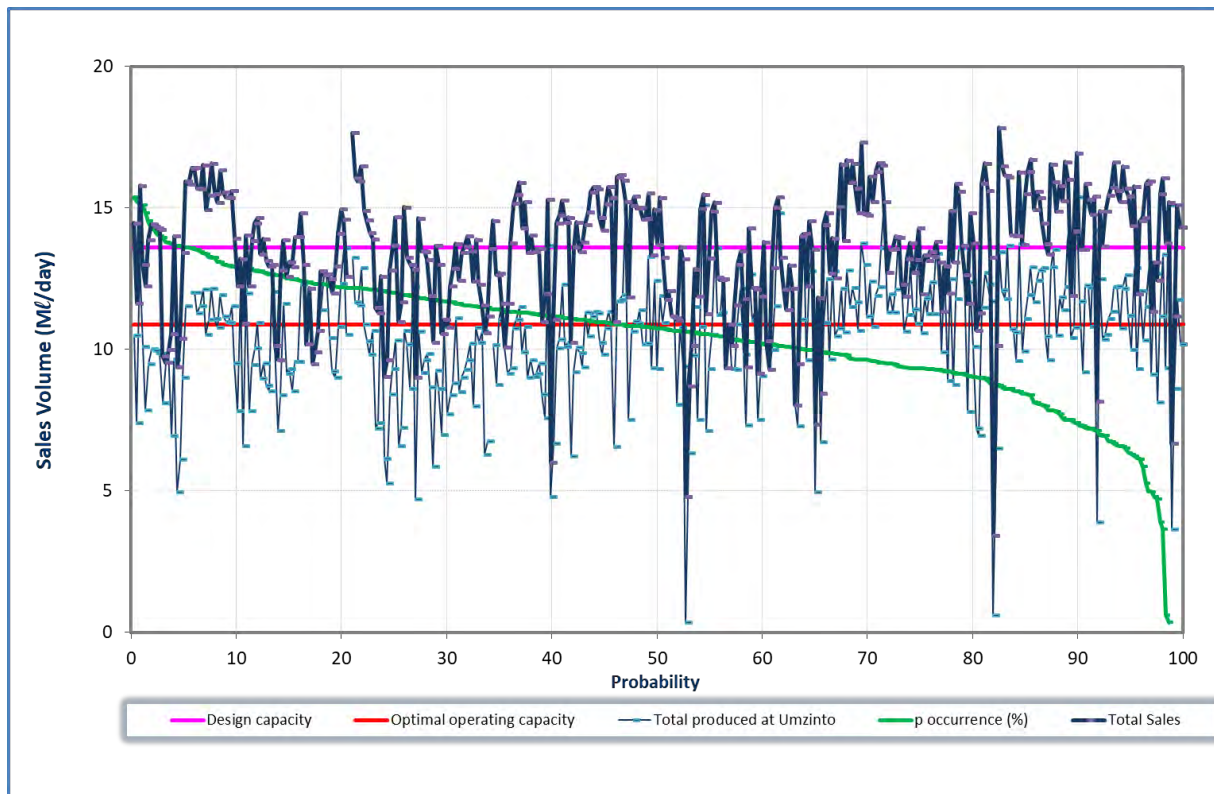
Figure 11.35 Analysis of historical production at Umzinto WTP (December 2024 to November 2025).
