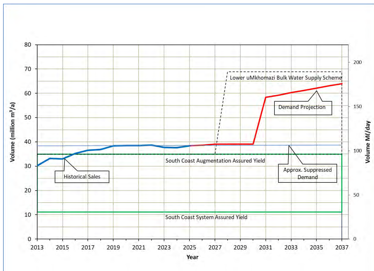
Figure 11.62 Upper and Middle South Coast water requirement projection scenarios.
