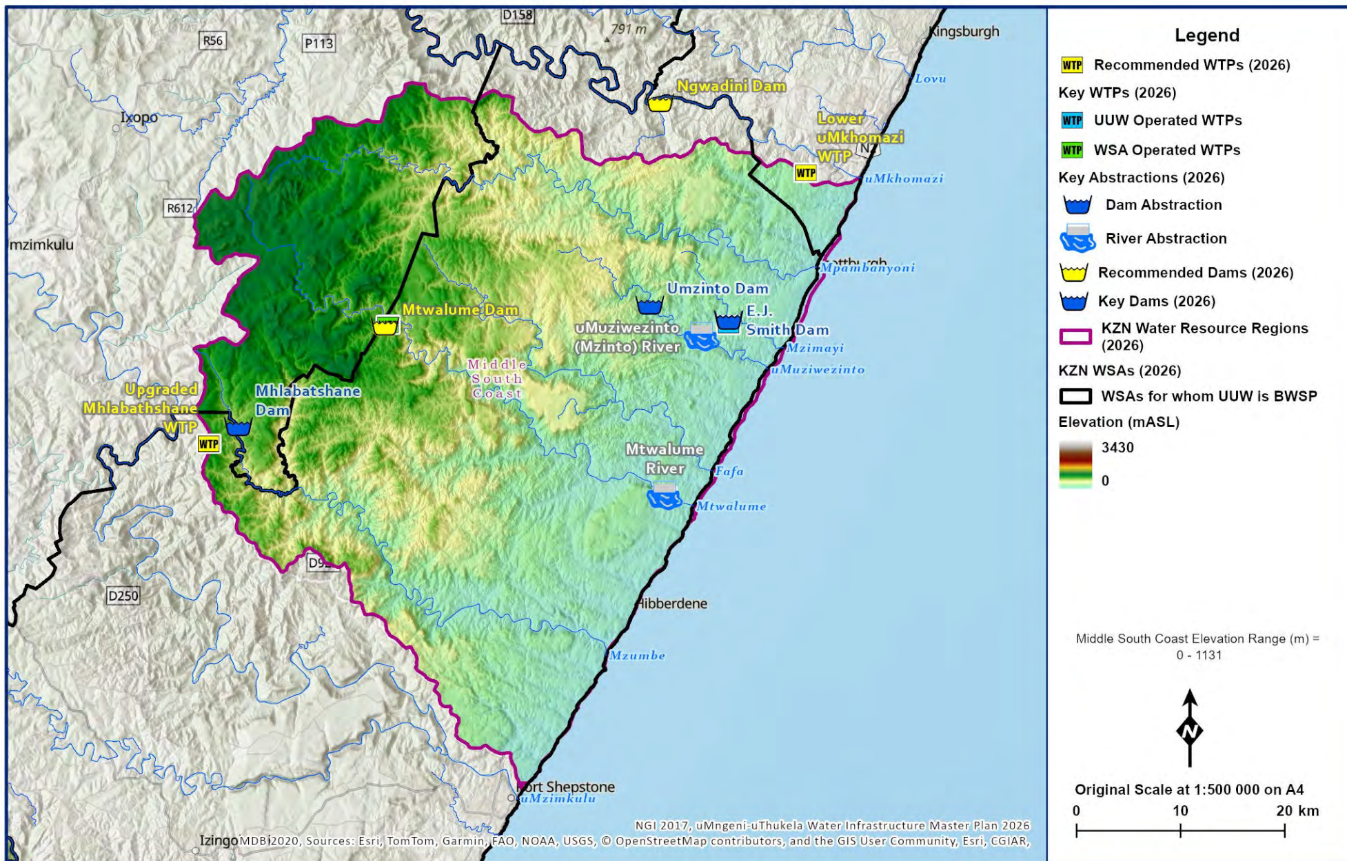
Figure 11.68 Proposed water resource infrastructure in the Middle South Coast Region.
