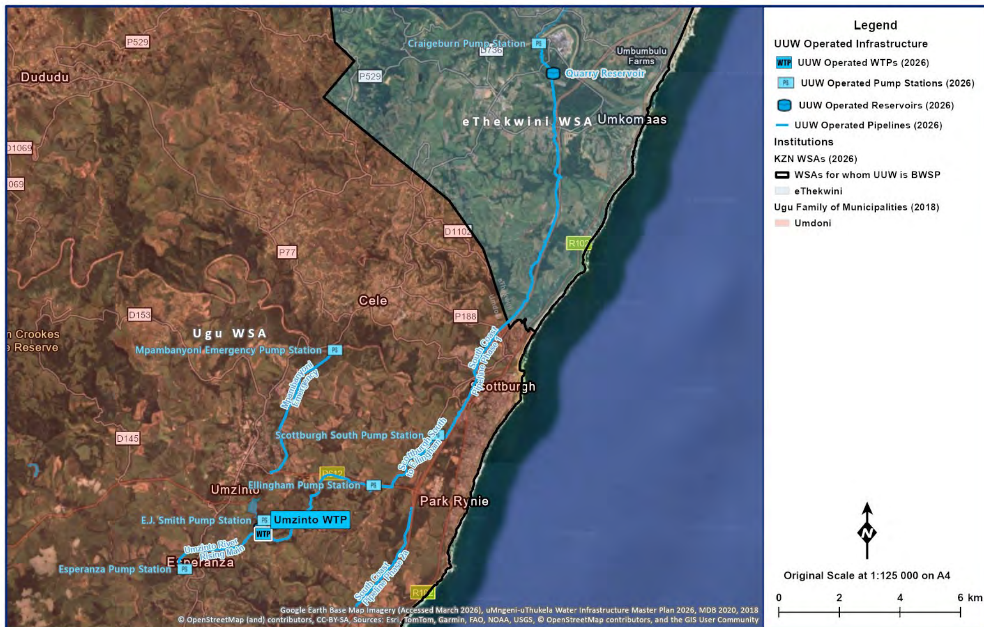
Figure 11.26 Umzinto Supply System.
