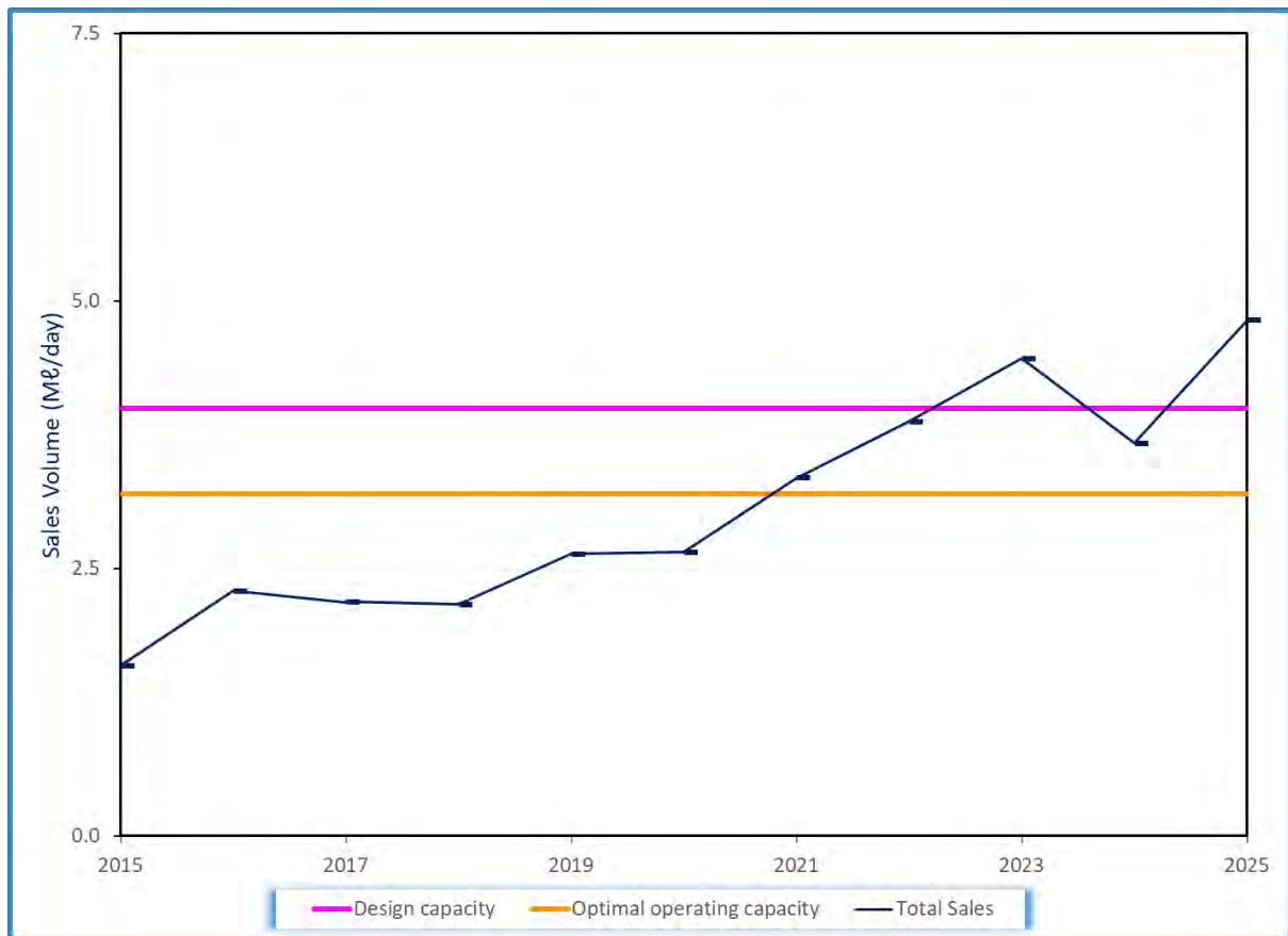
Figure 11.42 Analysis of historical production at Vulamehlo WTP (January 2015 to August 2025).
