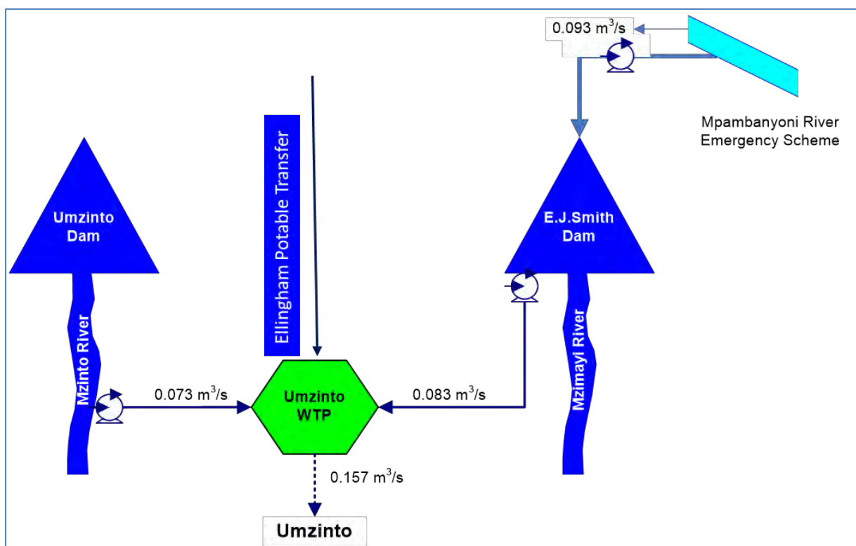
Figure 11.20 Schematic of the Middle South Coast system.
