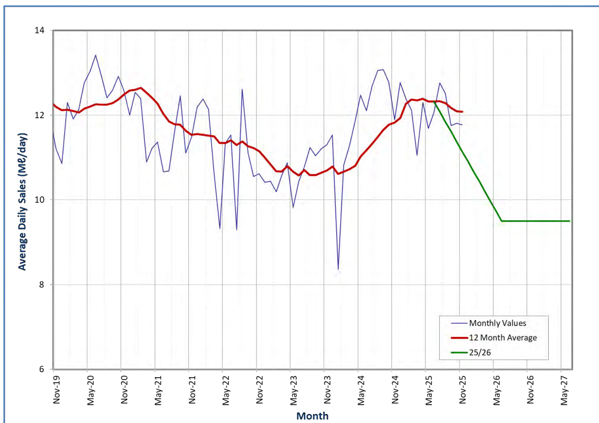
Figure 11.55 Water demand from Mtwalume WTP.
