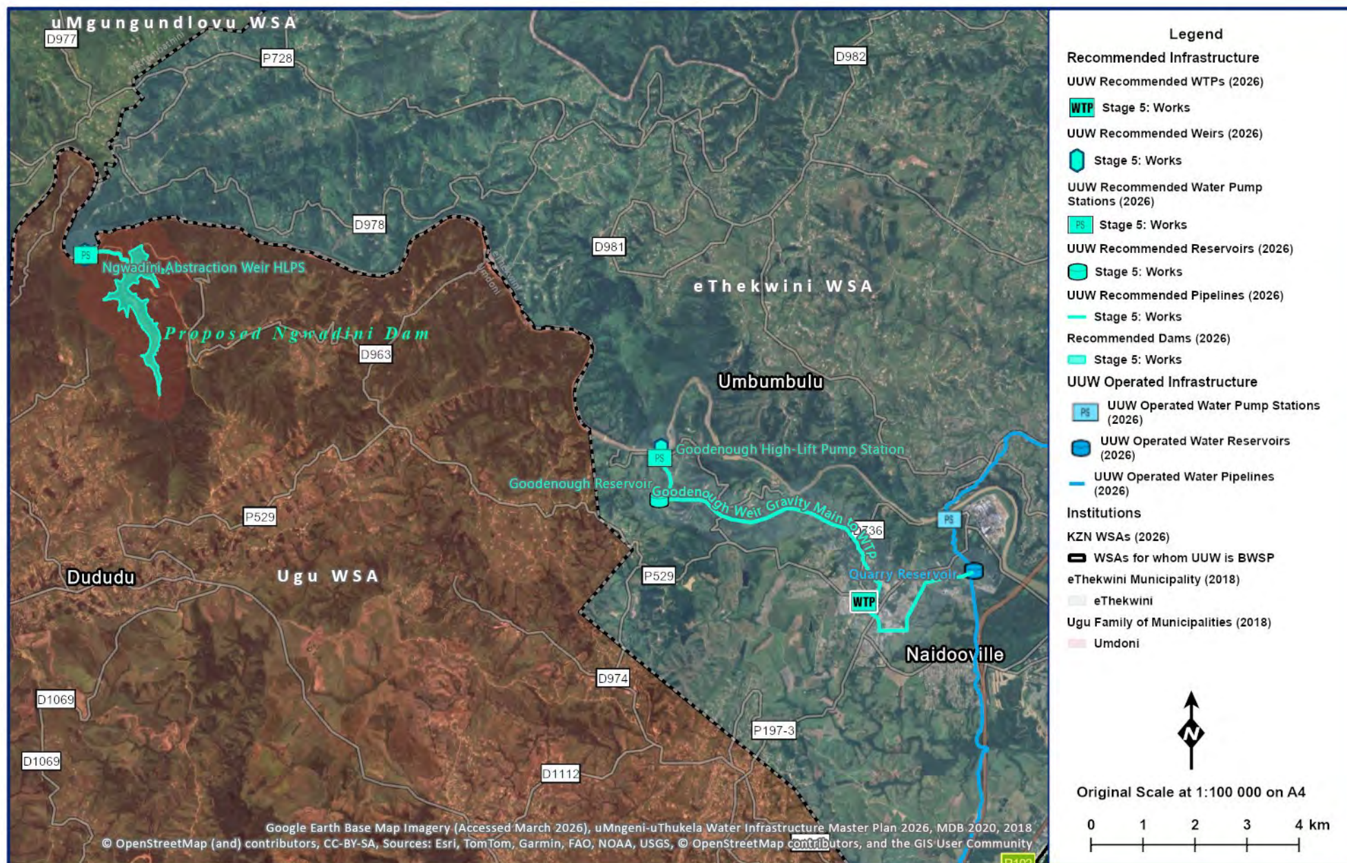
Figure 11.74 Layout of the proposed Lower uMkhomazi BWSS.
