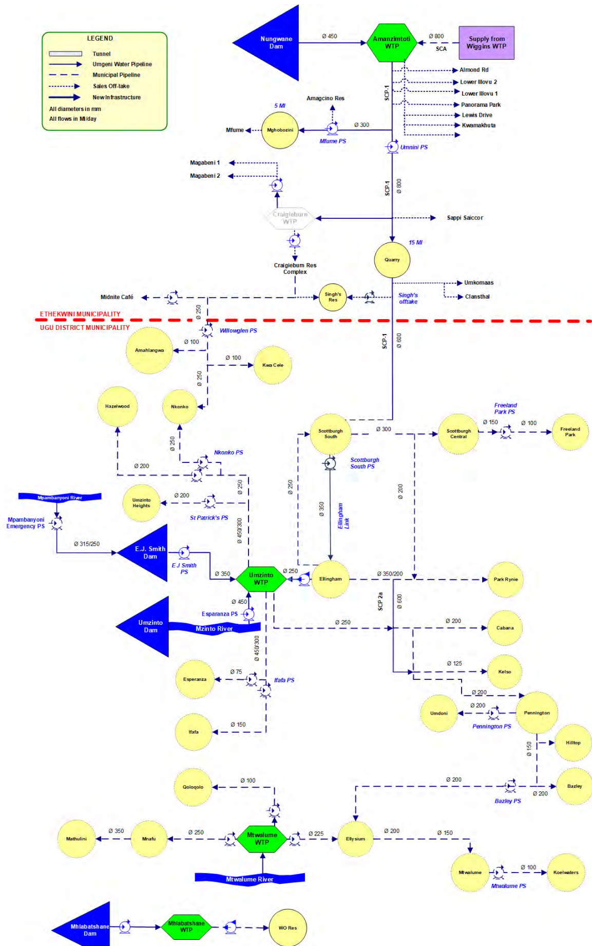
Figure 11.2 Schematic of the South Coast System (including Ugu District Municipality bulk supply infrastructure).
