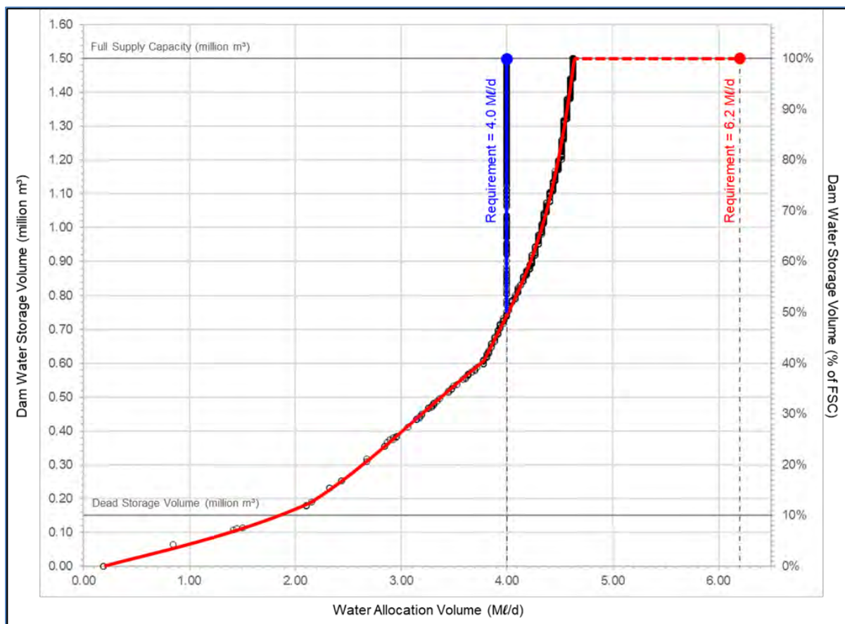
Figure 11.21 Mhlabatshane System Operating Rule (DWS, 2021)
