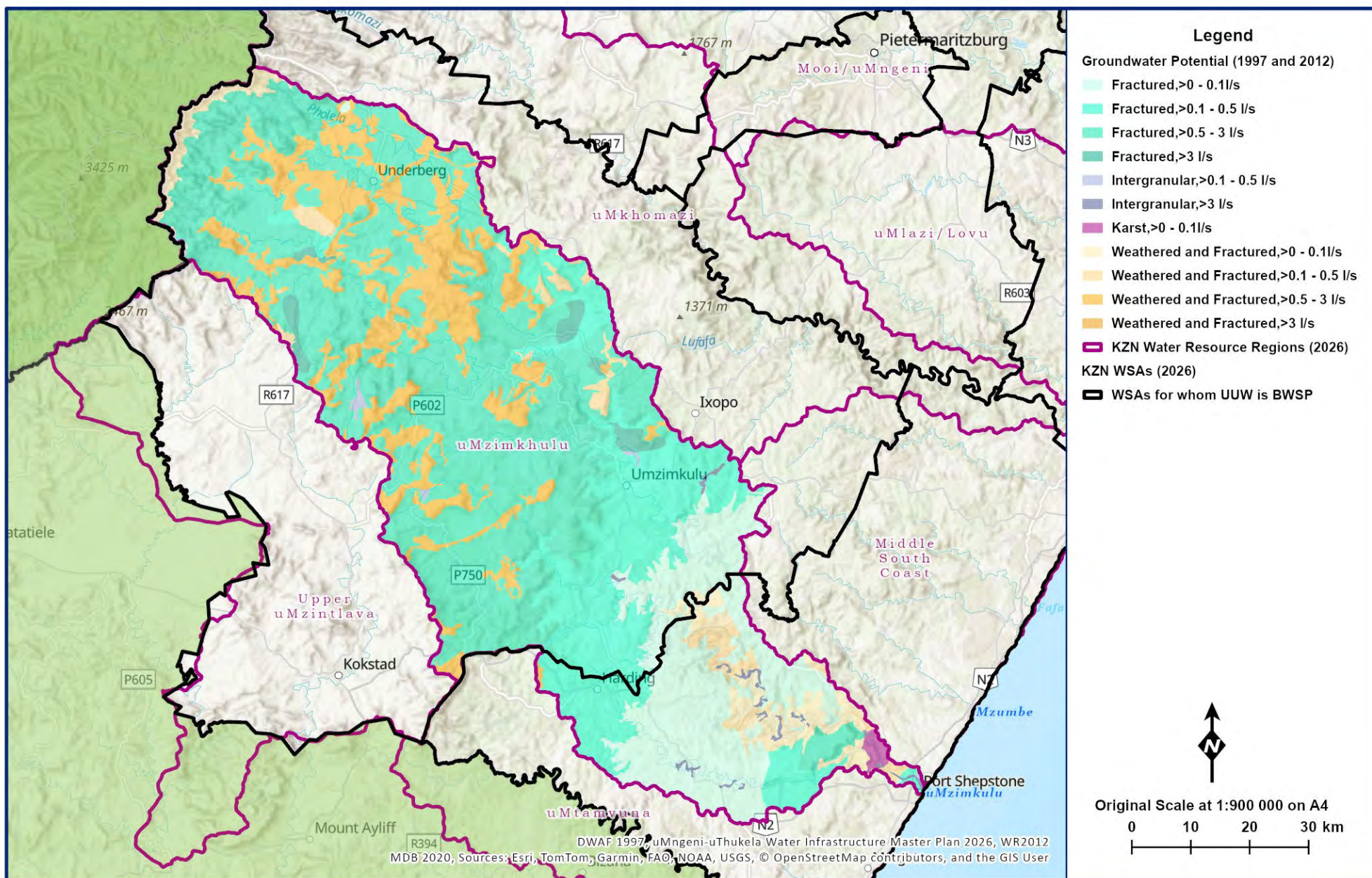
Figure 11.11 Groundwater potential in the uMzimkulu Region.
