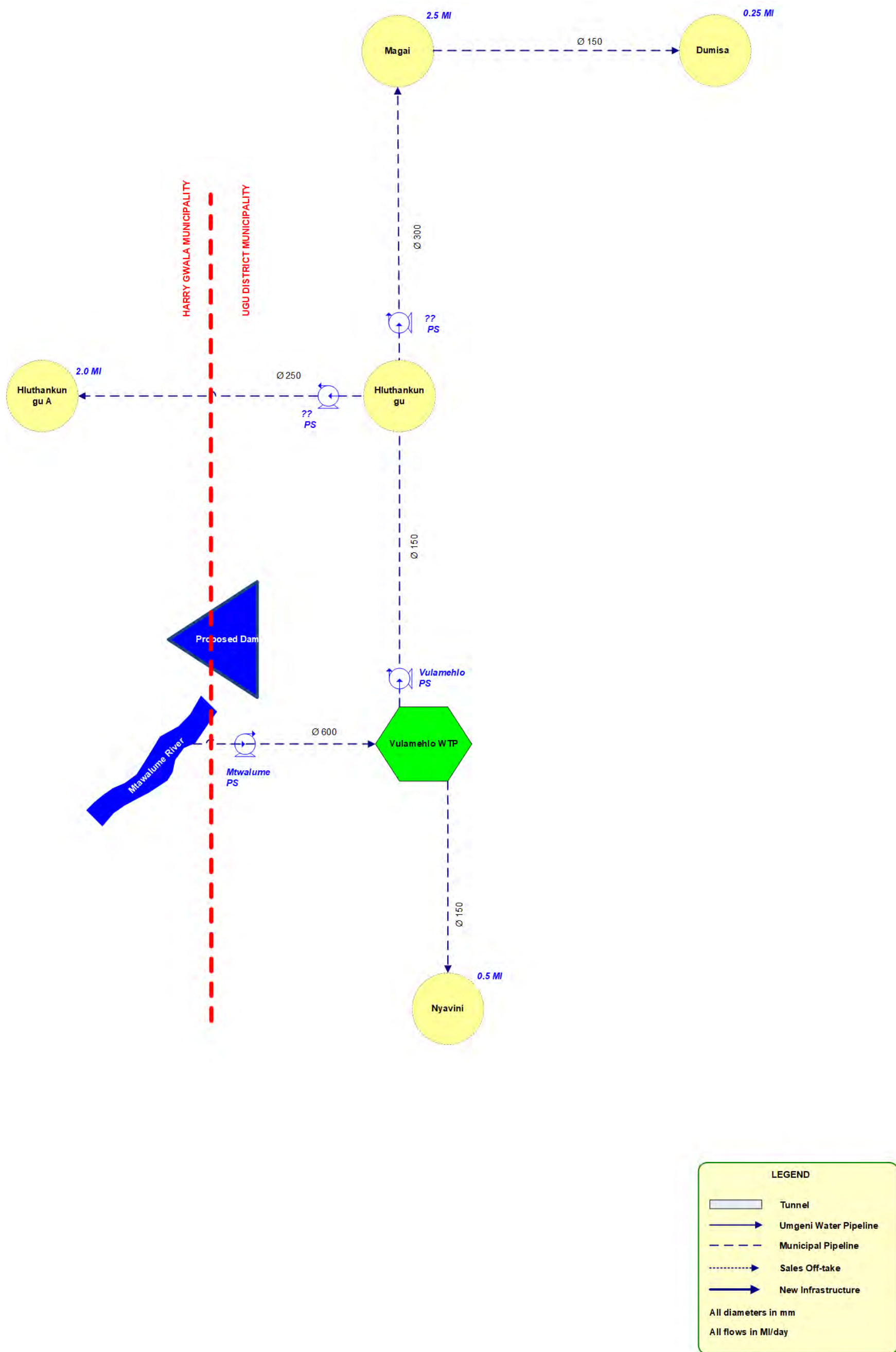
Figure 11.52 Schematic of the Vulamehlo System Bulk Supply Infrastructure.
