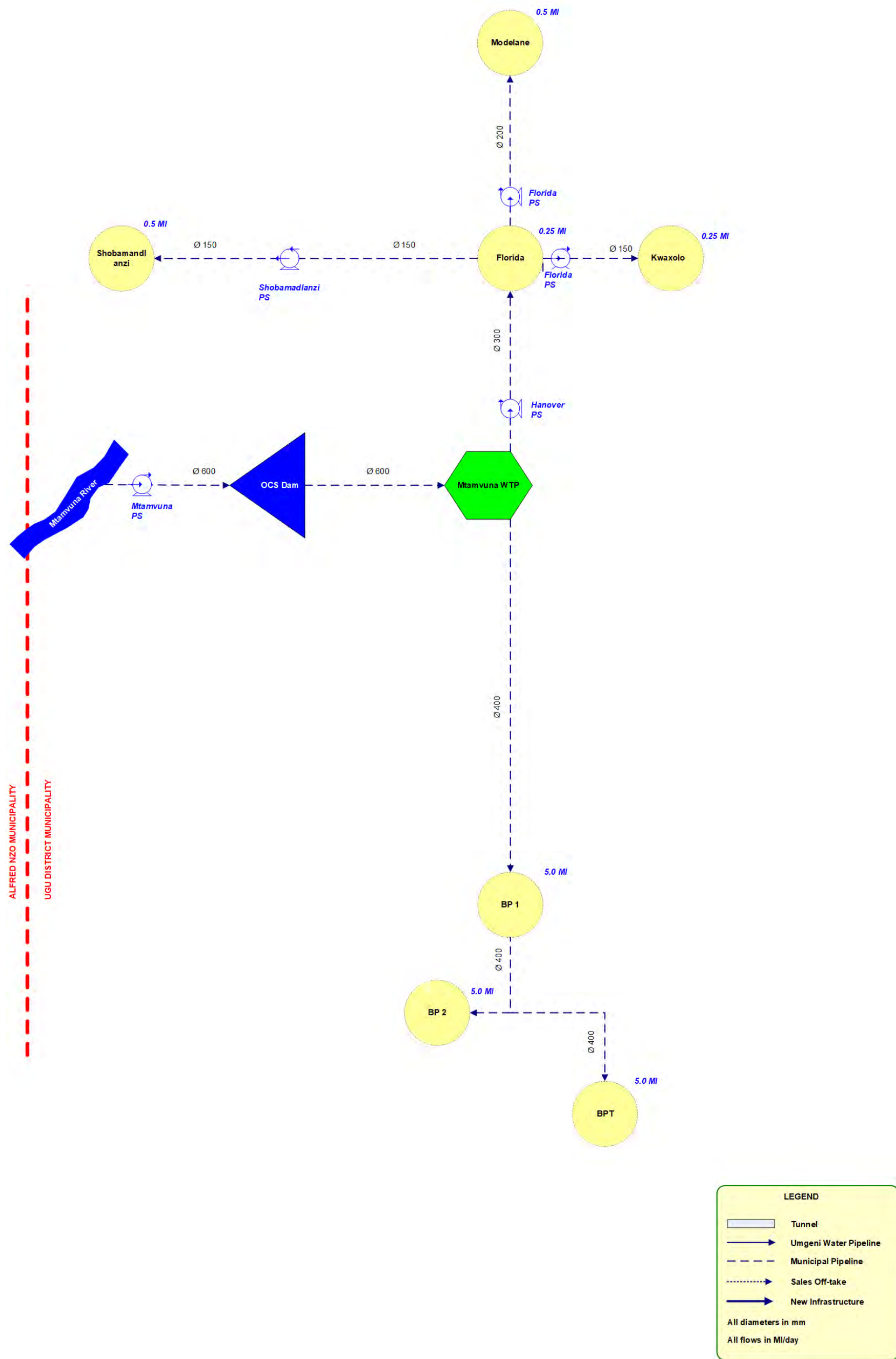
Figure 11.50 Schematic of the uMtavuna System Bulk Supply Infrastructure.
