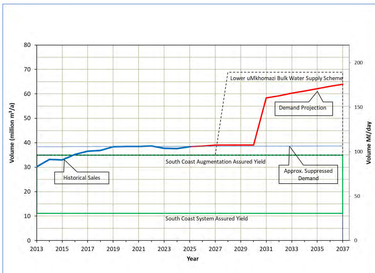
Figure 11.73 Water Balance Upper and Middle South Coast.
