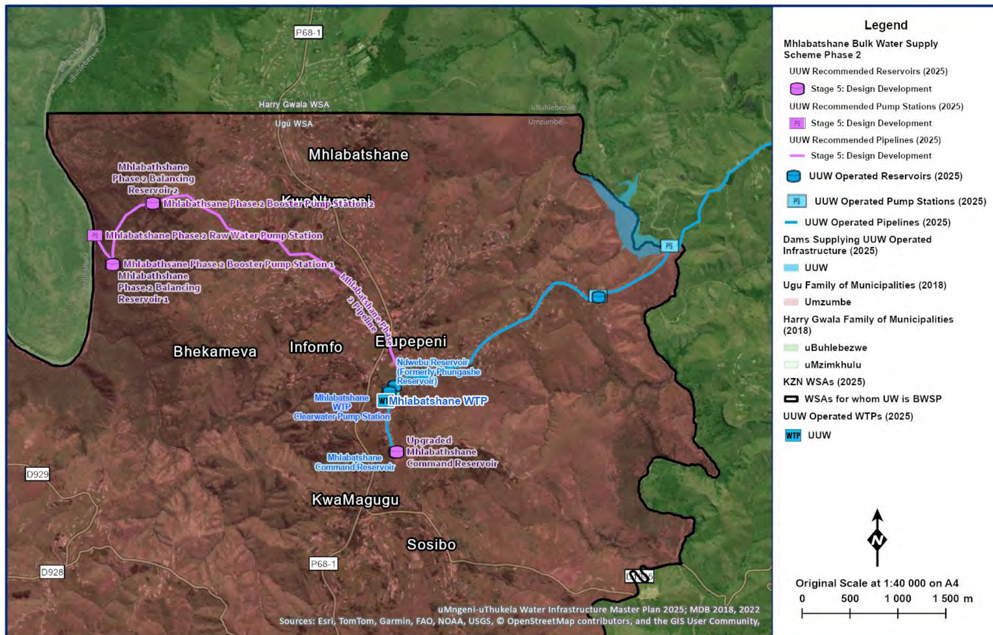
Figure 11.71 General layout of the Mhlabatshane BWSS Phase 2.
