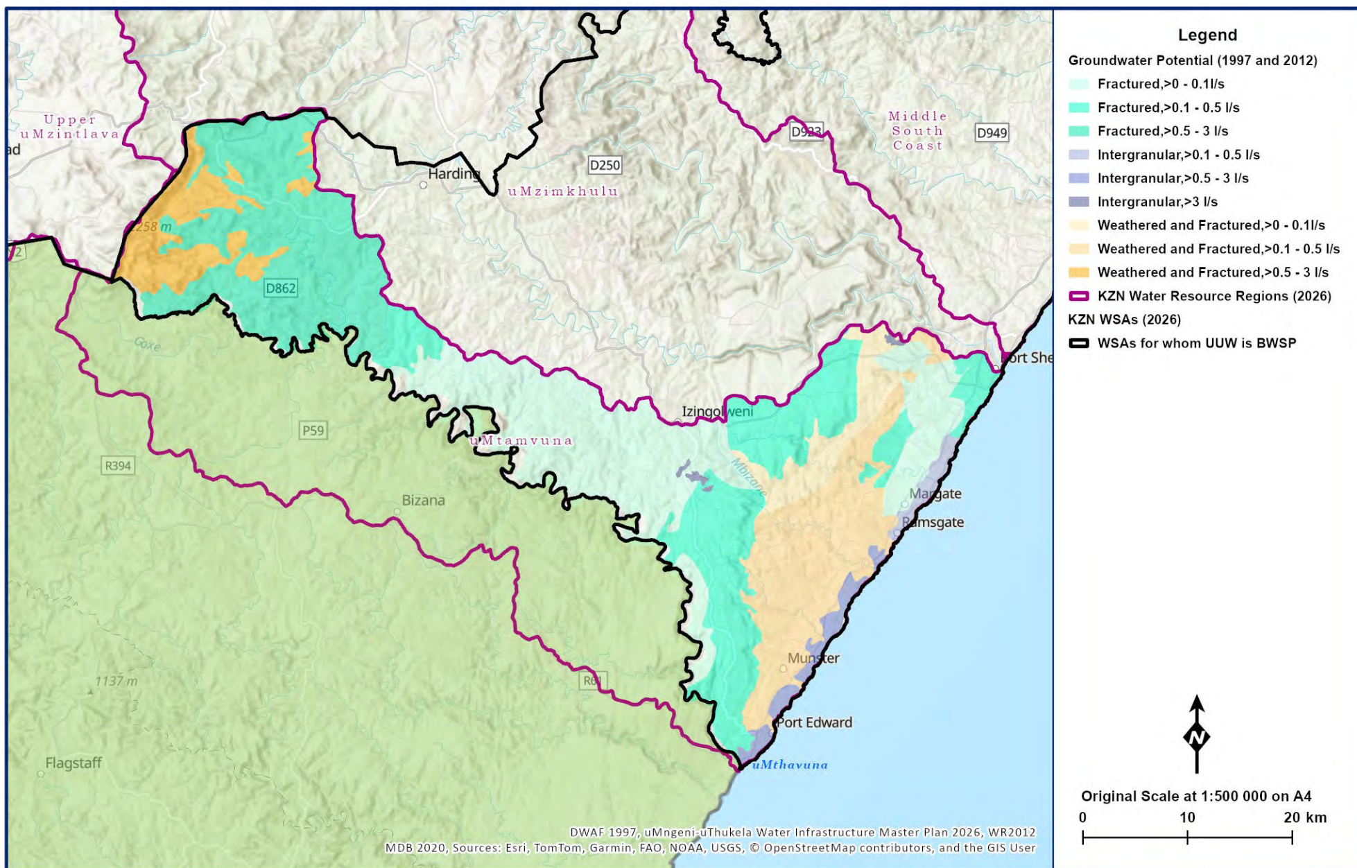
Figure 11.13 Groundwater potential in the uMthavuna Region.
