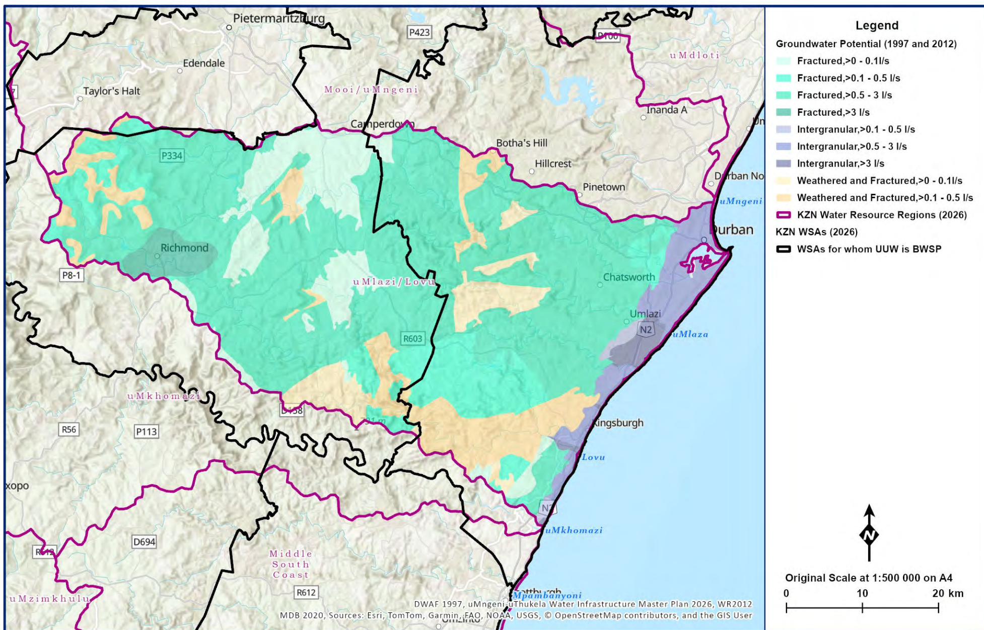
Figure 11.7 Groundwater potential in the Mlazi/Lovu Region.
