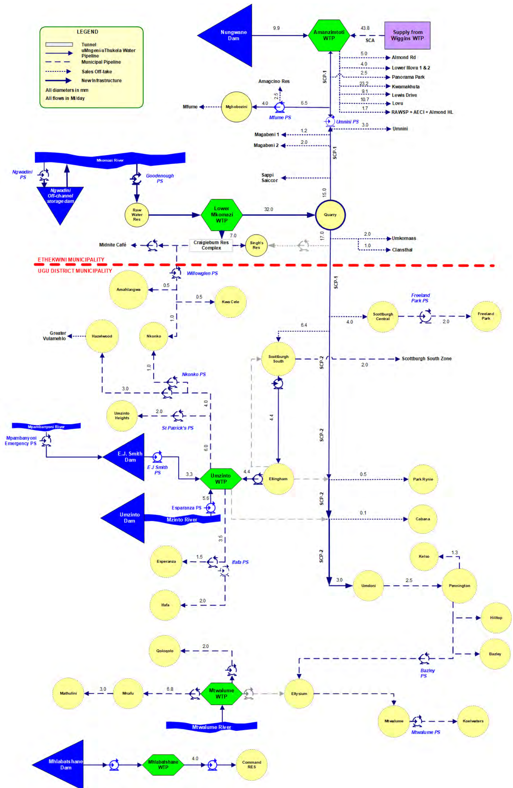
Figure 11.44 Five year demand projection for the South Coast System.
