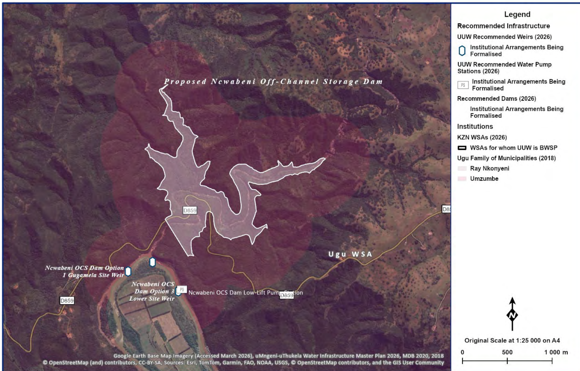
Figure 11.77 General layout of the Ncwabeni OCS Dam and Abstraction Work.
