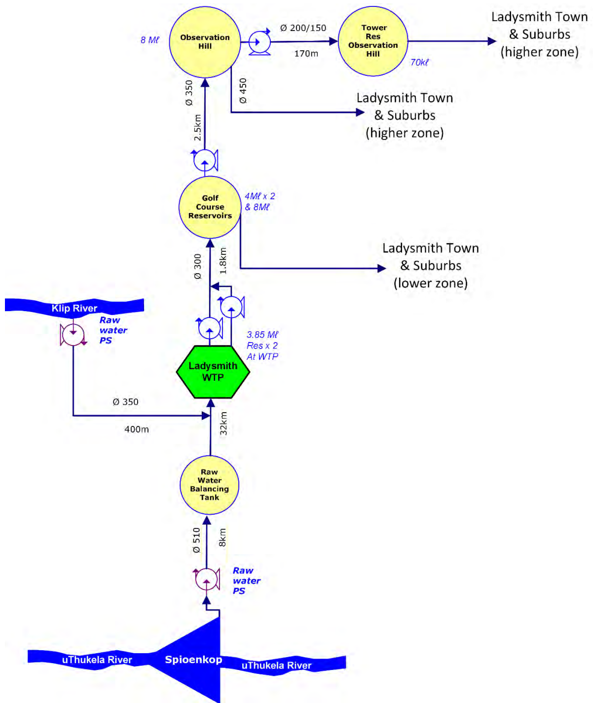
Figure 13.58 Ladysmith WTP Supply System Schematic (not to scale; uTDM Infrastructure)
