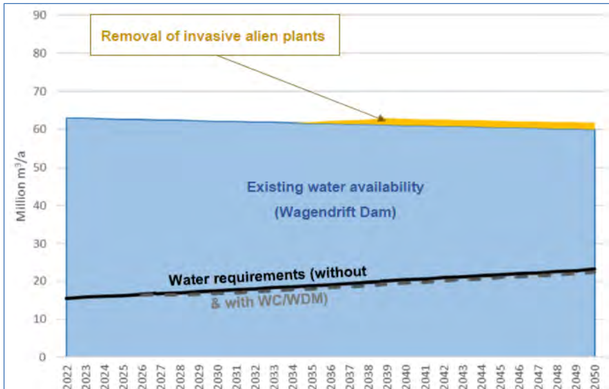
Figure 13.73 Water Balance for the Bushmans System (DWS 2024)
