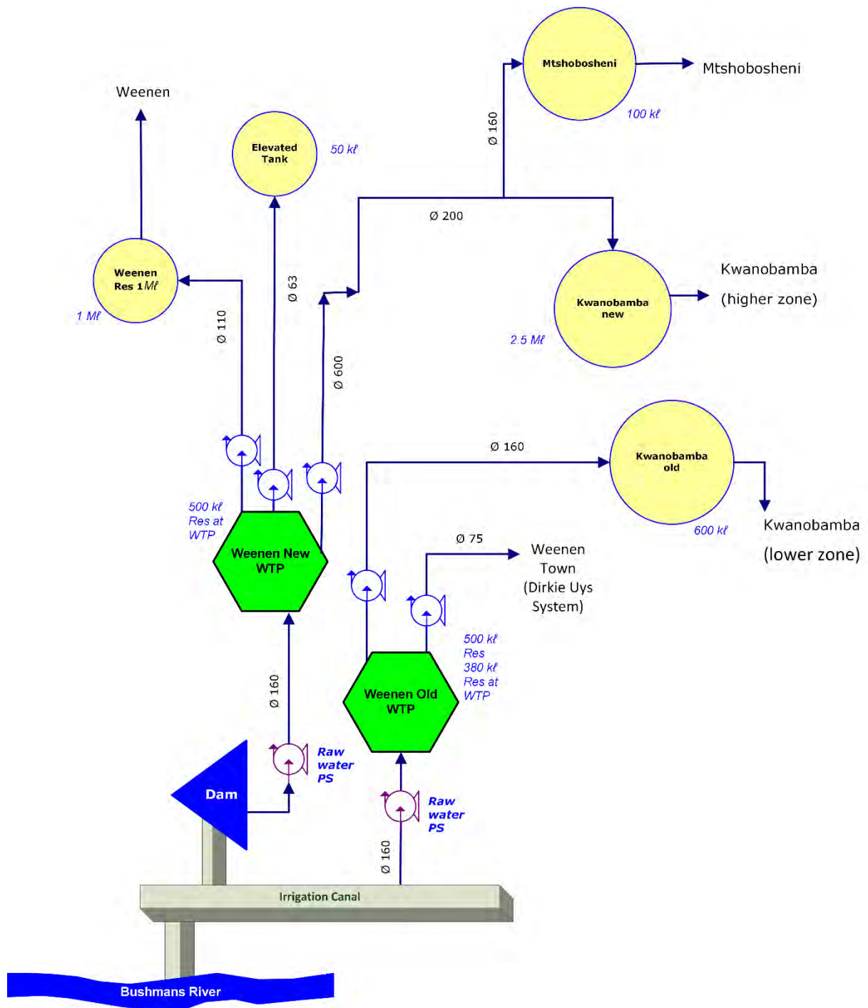
Figure 13.67 Weenen WTP (Old WTP and New WTP) Supply System Schematic (not to scale; uTDM Infrastructure)
