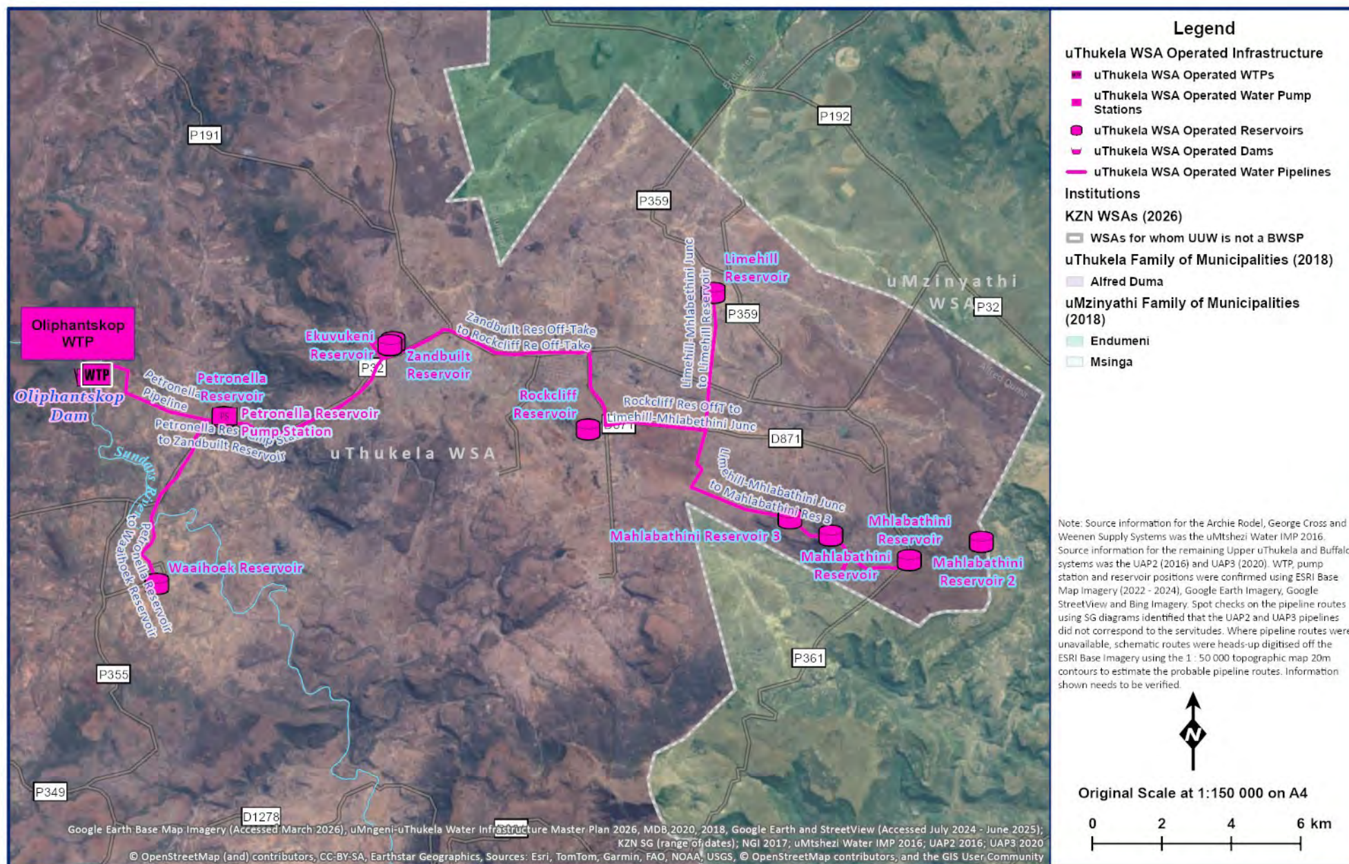
Figure 13.37 Olifantskop WTP Supply System layout.
