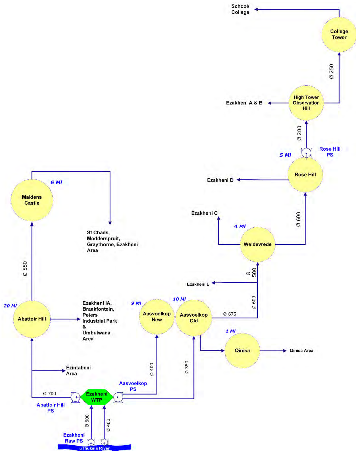
Figure 13.23 Ezakheni WTP Supply System schematic.
