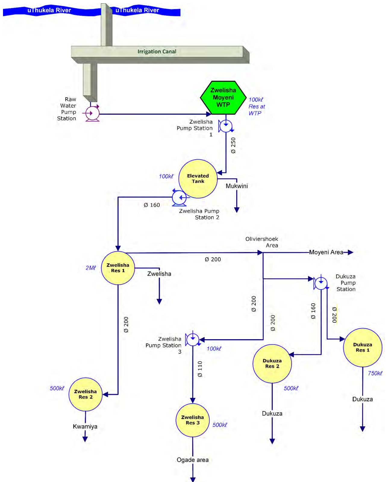
Figure 13.49 Zwelisha Moyeni WTP Supply System Schematic (not to scale; uTDM Infrastructure)
