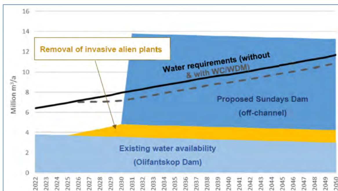
Figure 13.72 Water balance for the Sundays System (DWS 2024).
