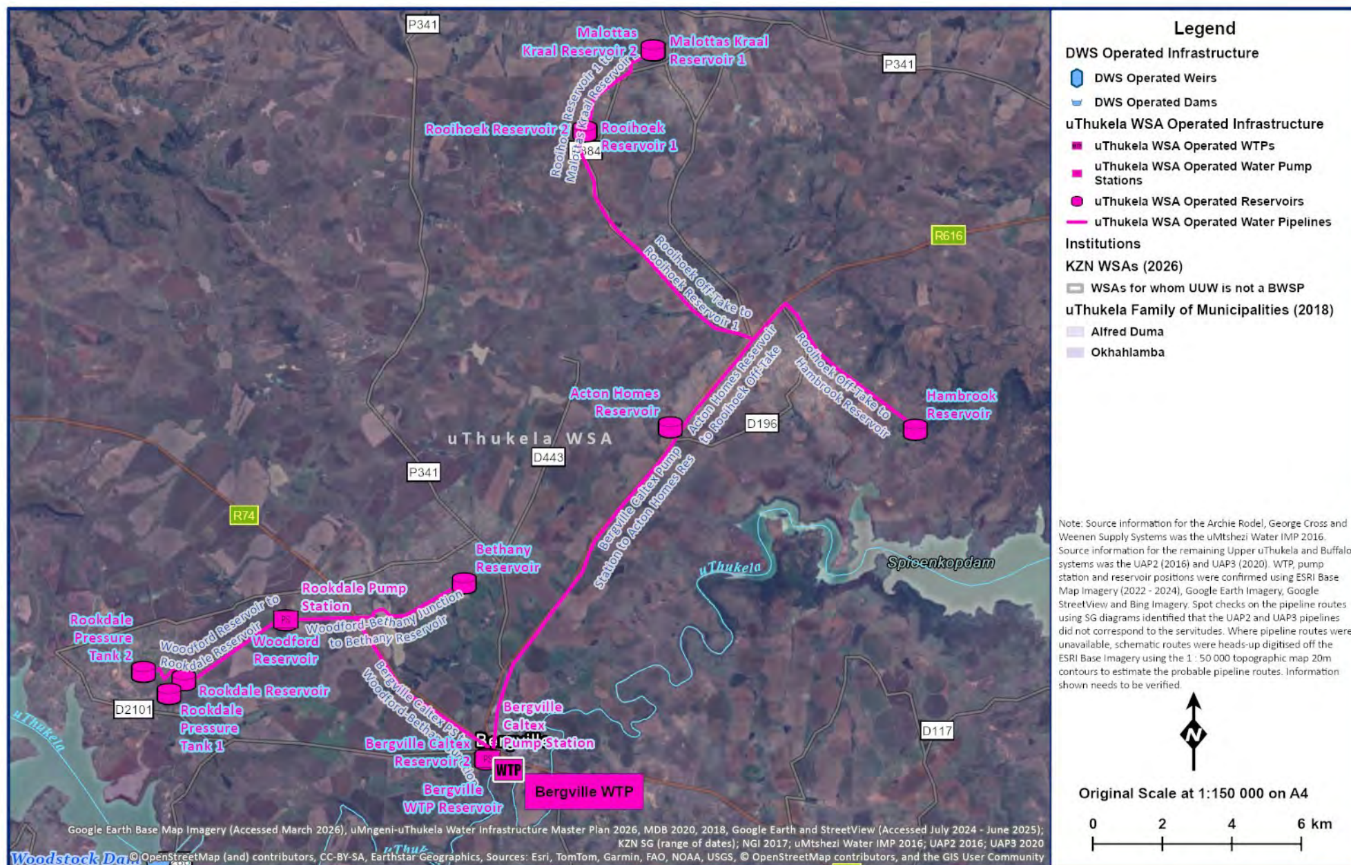
Figure 13.51 Bergville WTP Supply System Layout.
