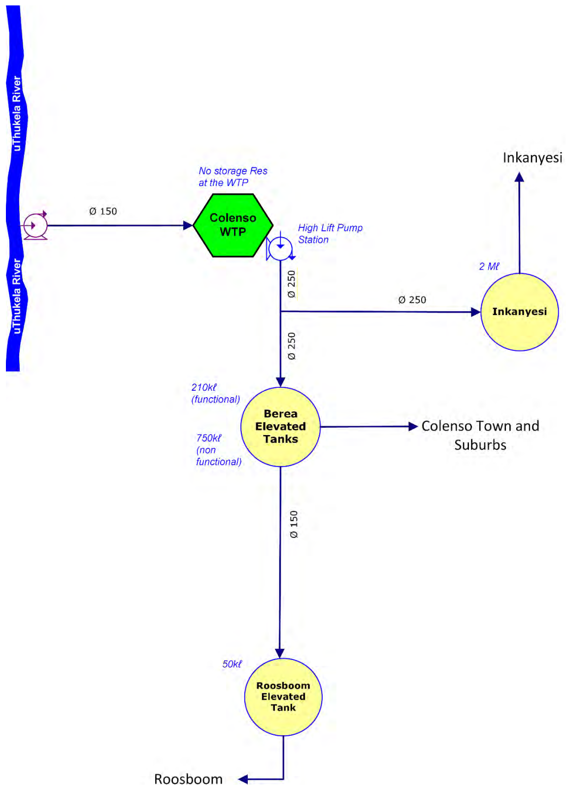
Figure 13.55 Colenso WTP Supply System Schematic (not to scale; uTDM Infrastructure)
