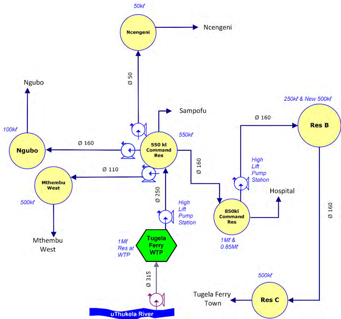
Figure 13.70 Tugela Ferry WTP Supply System Schematic (not to scale; uMzinyathi DM Infrastructure)
