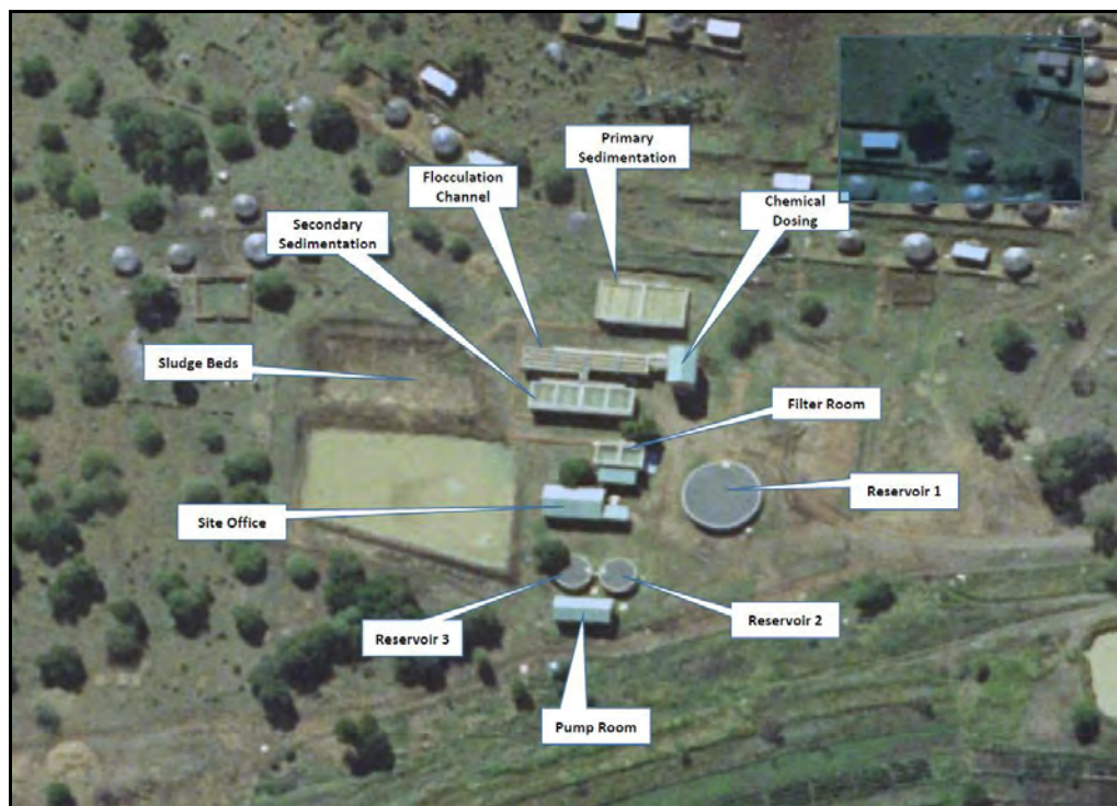
Figure 13.68 Overview of Tugela Ferry WTP, uMzinyathi DM O&M Manual (December 2016)
