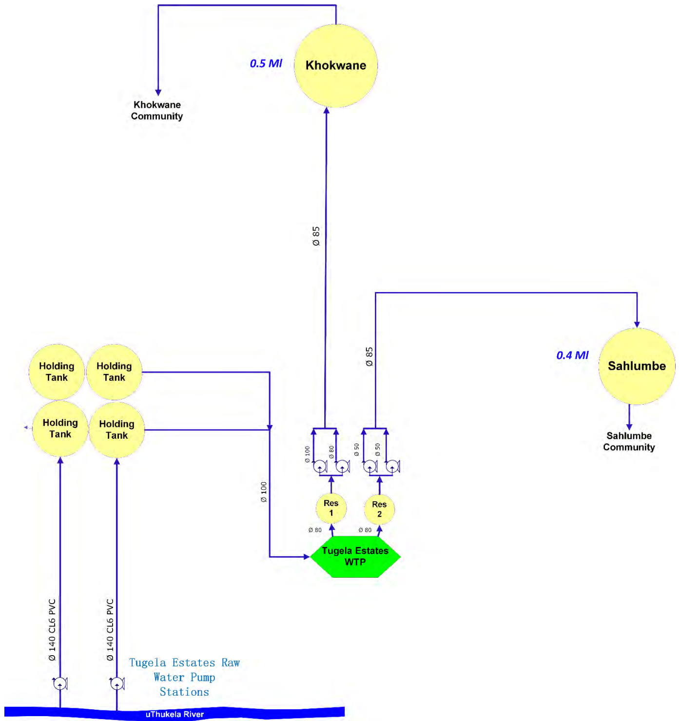
Figure 13.33 Tugela Estates WTP Supply System schematic.
