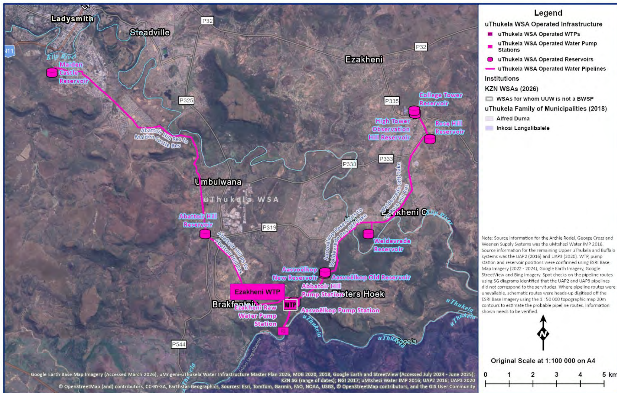
Figure 13.22 Ezakheni WTP Supply System layout.
