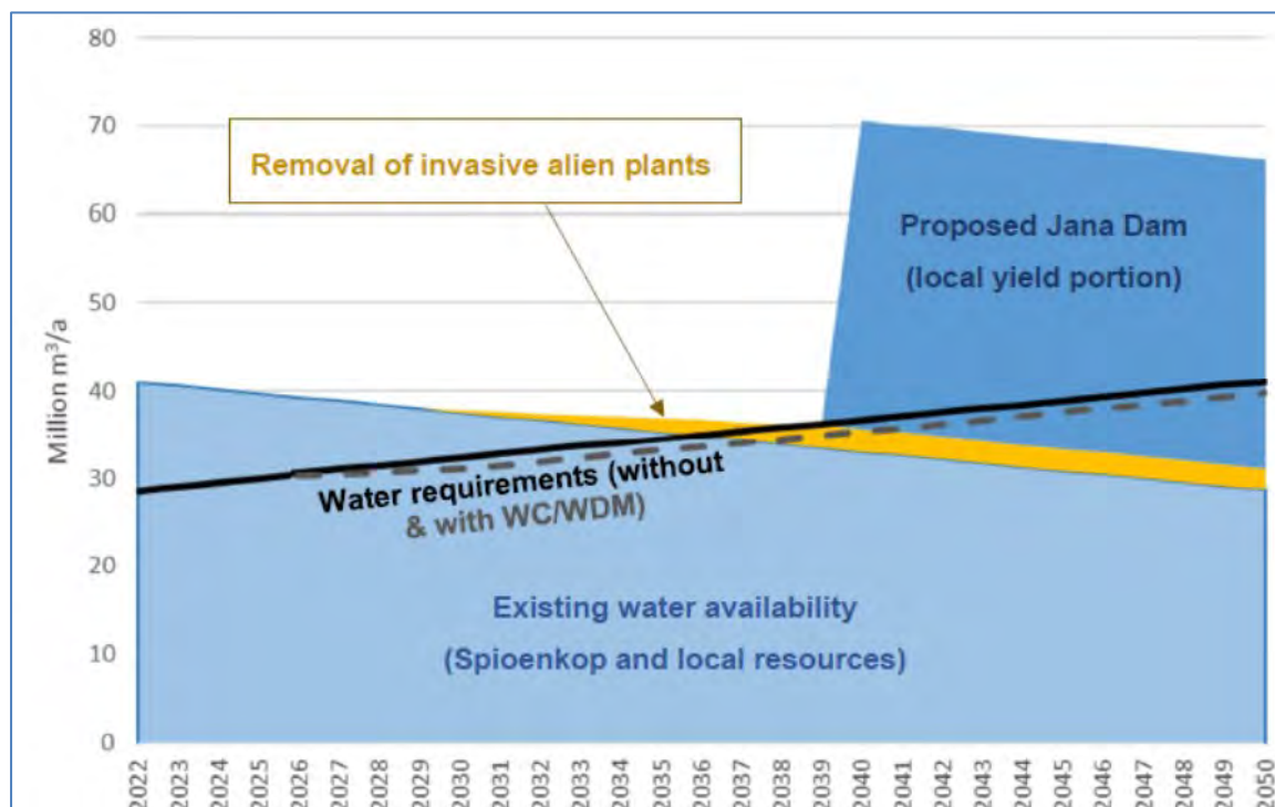
Figure 13.71 Water balance for the Upper Thukela Supply system (DWS 2024).
