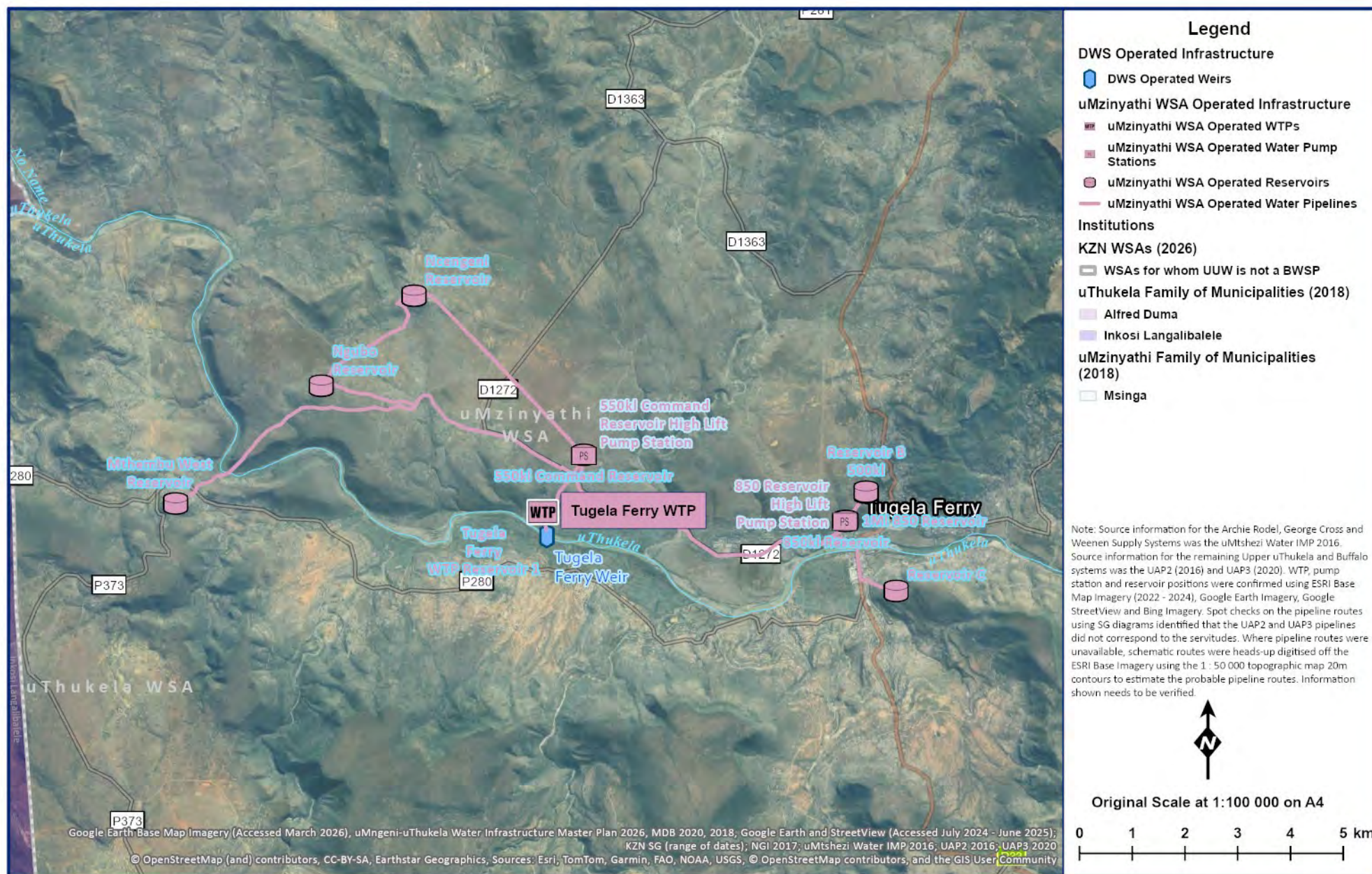
Figure 13.69 Tugela Ferry WTP Supply System Layout.
