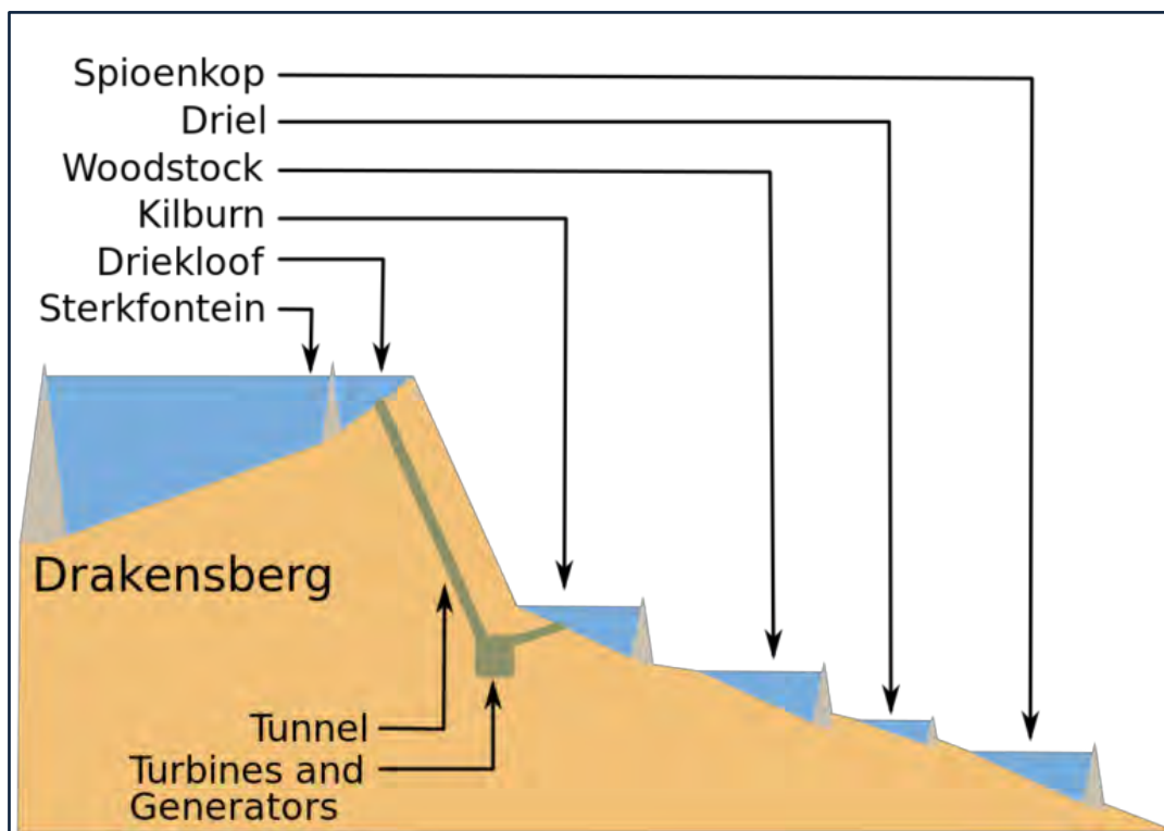
Figure 13.20 Longitudinal profile of the Thukela-Vaal Scheme and the Drakensberg Pumped Storage Scheme (Ladysmith Gazette 2017: website 15 ).
