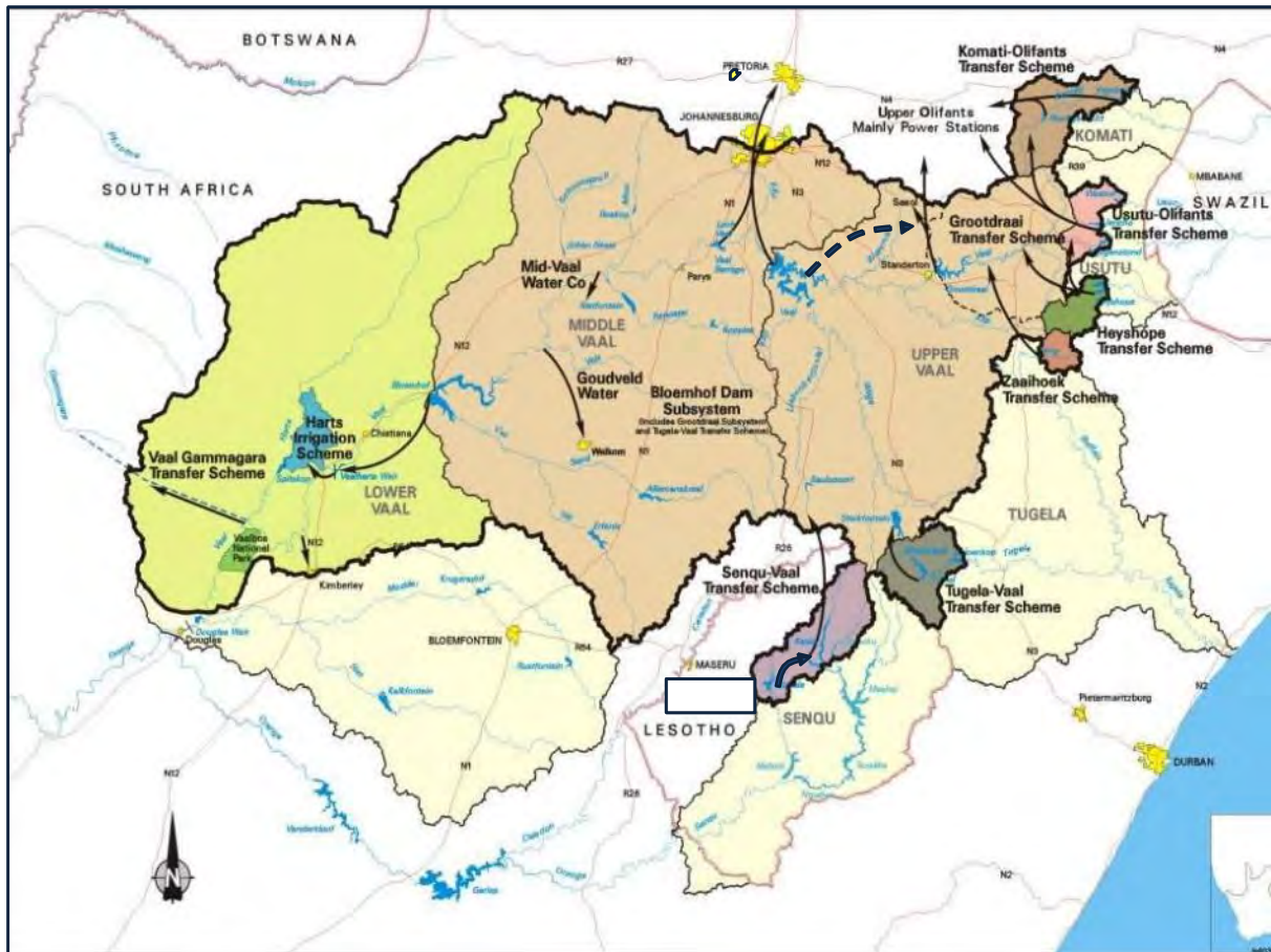
Figure 13.16 The Thukela-Vaal Transfer Scheme in the Vaal River System (DWS 2018: Slide 6).
