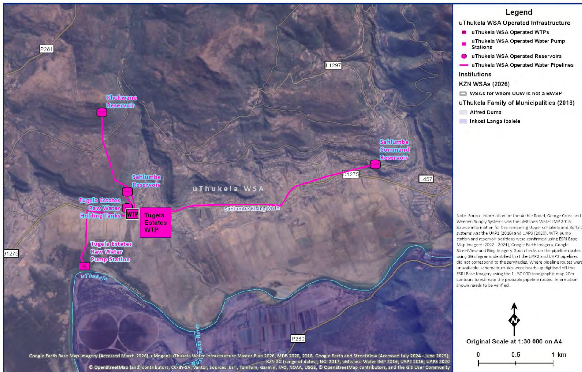
Figure 13.26 Tugela Estates WTP and uMhlamayo Borehole Supply System layout.
