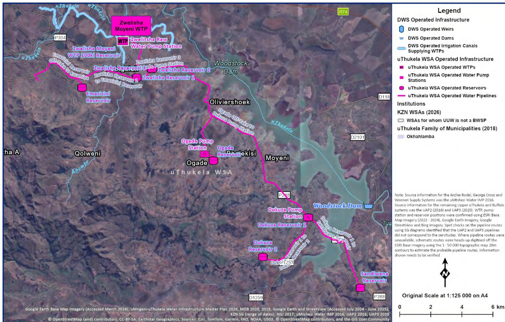
Figure 13.48 Zwelisha Moyeni WTP Supply System Layout.
