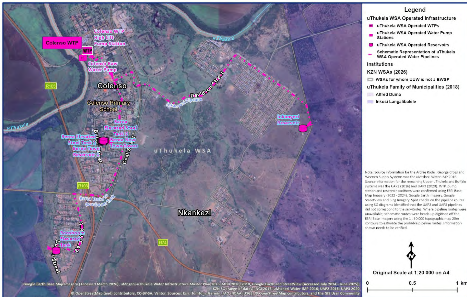
Figure 13.54 Colenso WTP Supply System Layout.
