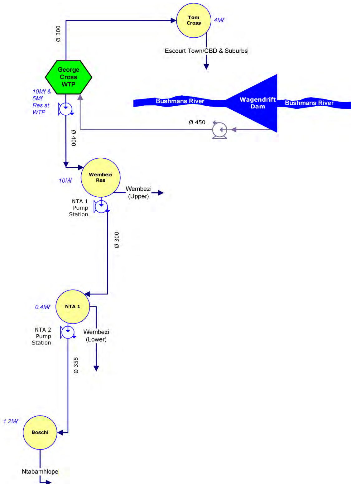
Figure 13.64 George Cross WTP Supply System Schematic (not to scale; uTDM Infrastructure)
