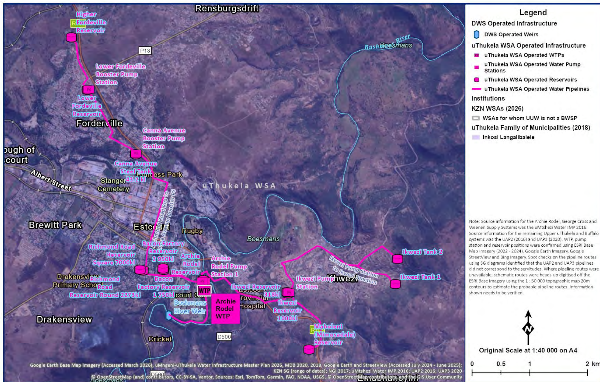
Figure 13.60 Archie Rodel (Estcourt) WTP Supply System.
