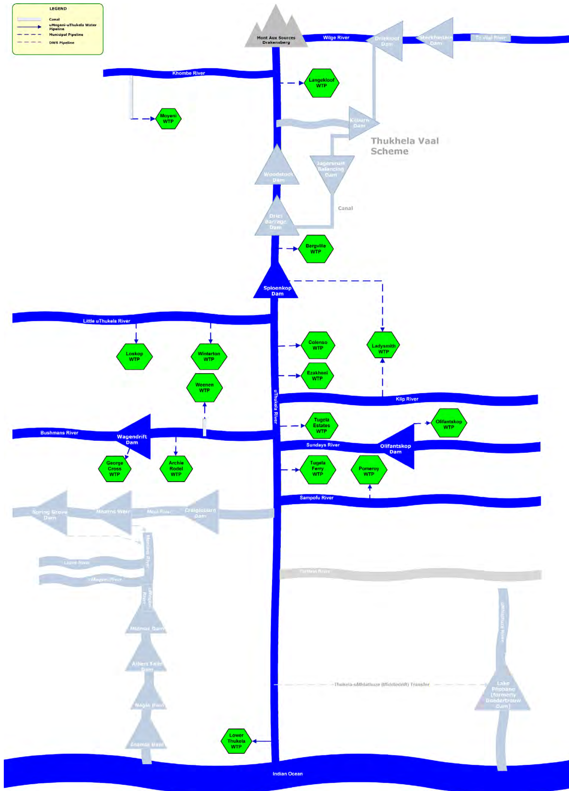
Figure 13.1 Schematic of the uThukela River System with key abstractions (excluding the Buffalo River)
