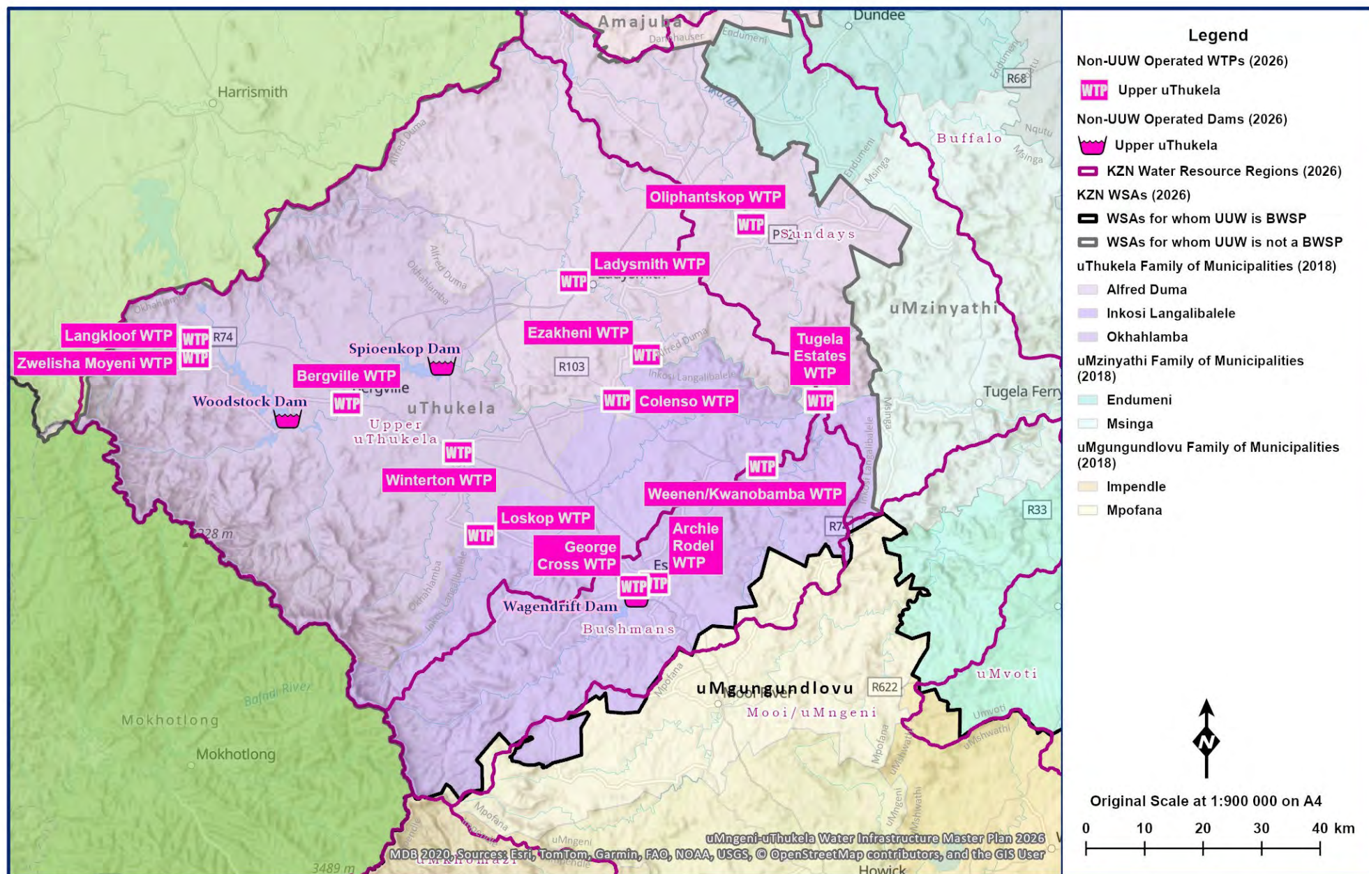
Figure 13.3 General layout of the Upper uThukela System.
