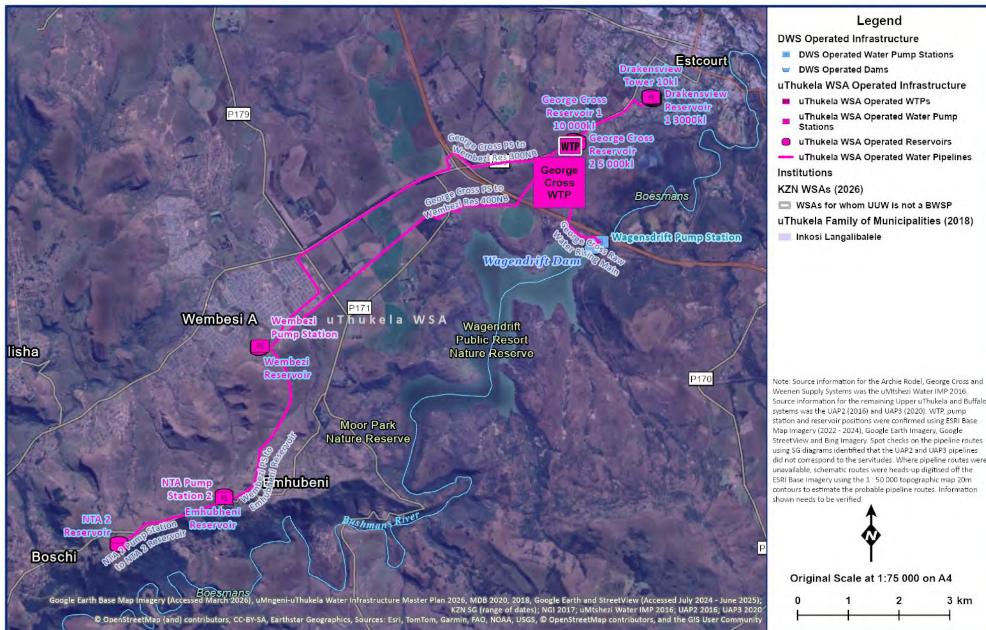
Figure 13.63 George Cross WTP (Estcourt) WTP Supply System Layout.
