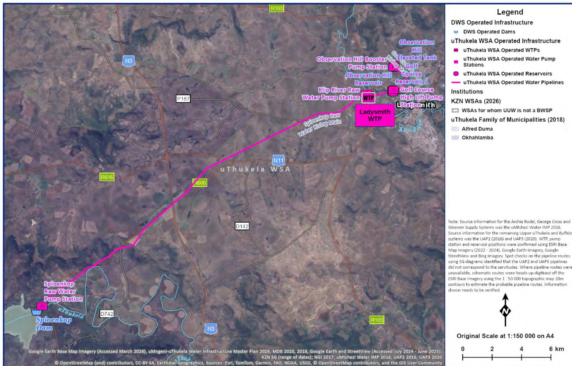
Figure 13.57 Ladysmith WTP Supply System Layout.
