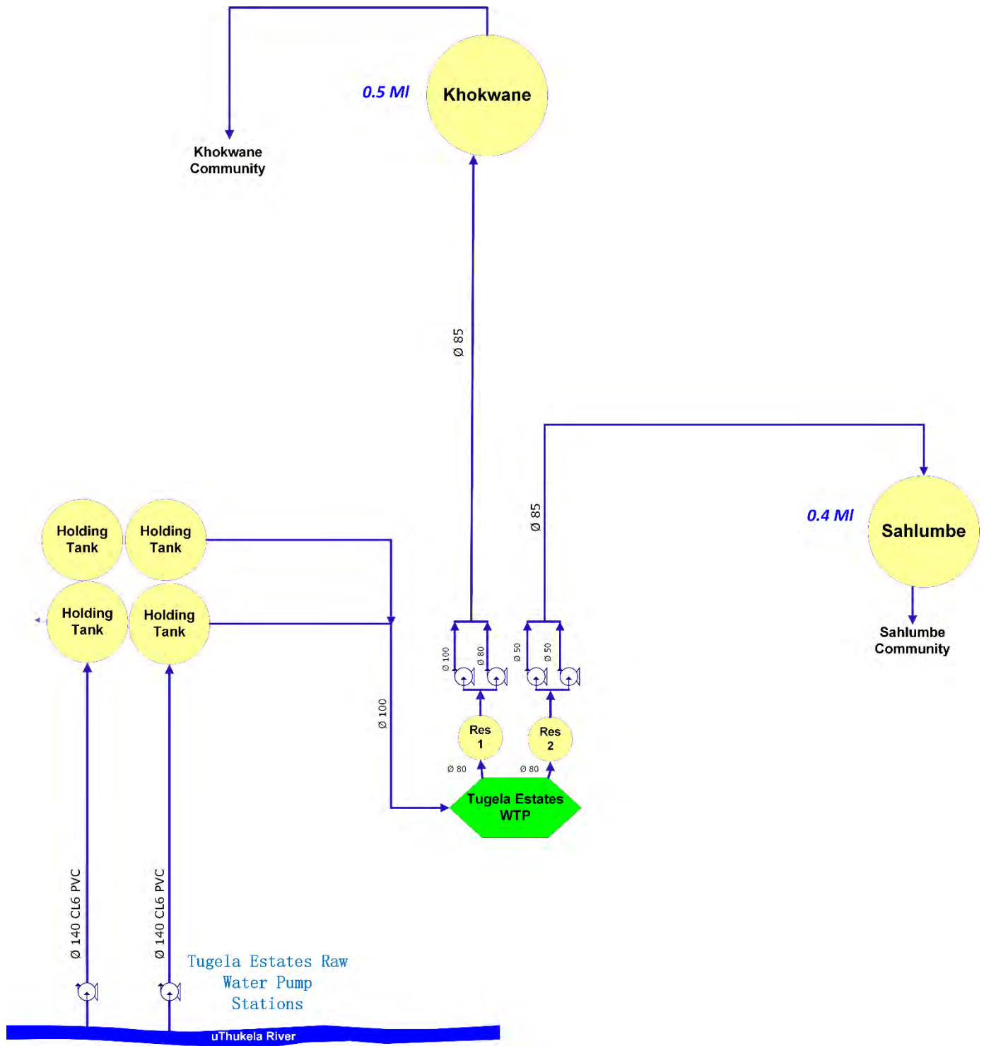
Figure 13.33 Tugela Estates WTP Supply System schematic.
