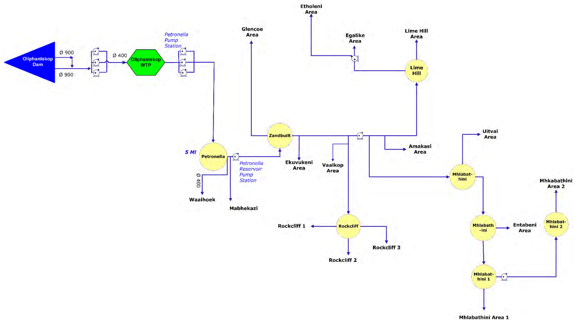
Figure 13.38 Olifantskop WTP Supply System schematic.
