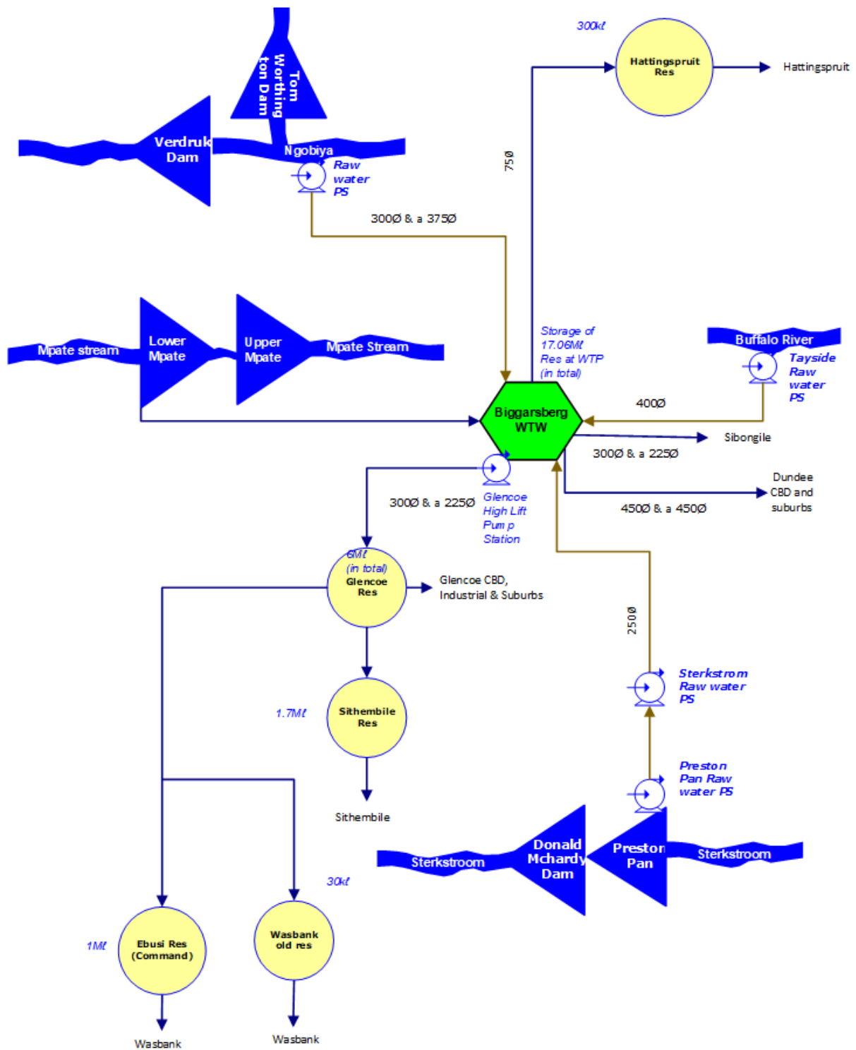
Figure 14.47 Biggarsberg WTP Supply Schematic (not to scale; uMzinyathi bulk infrastructure)
