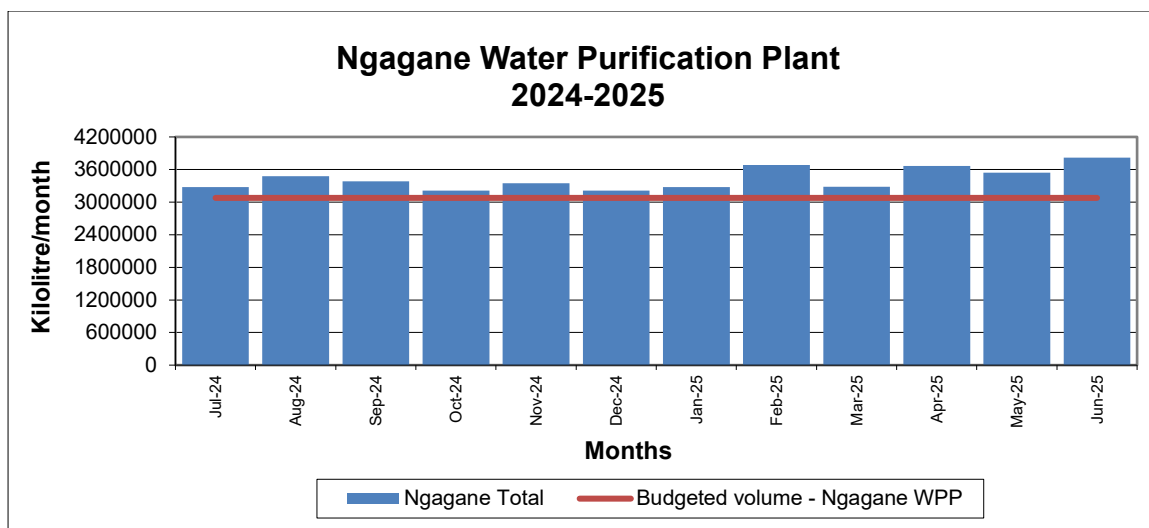
Figure 14.56 Output of Ngagane WTP in 2024/2025 FY (uThukela Water 2026)
