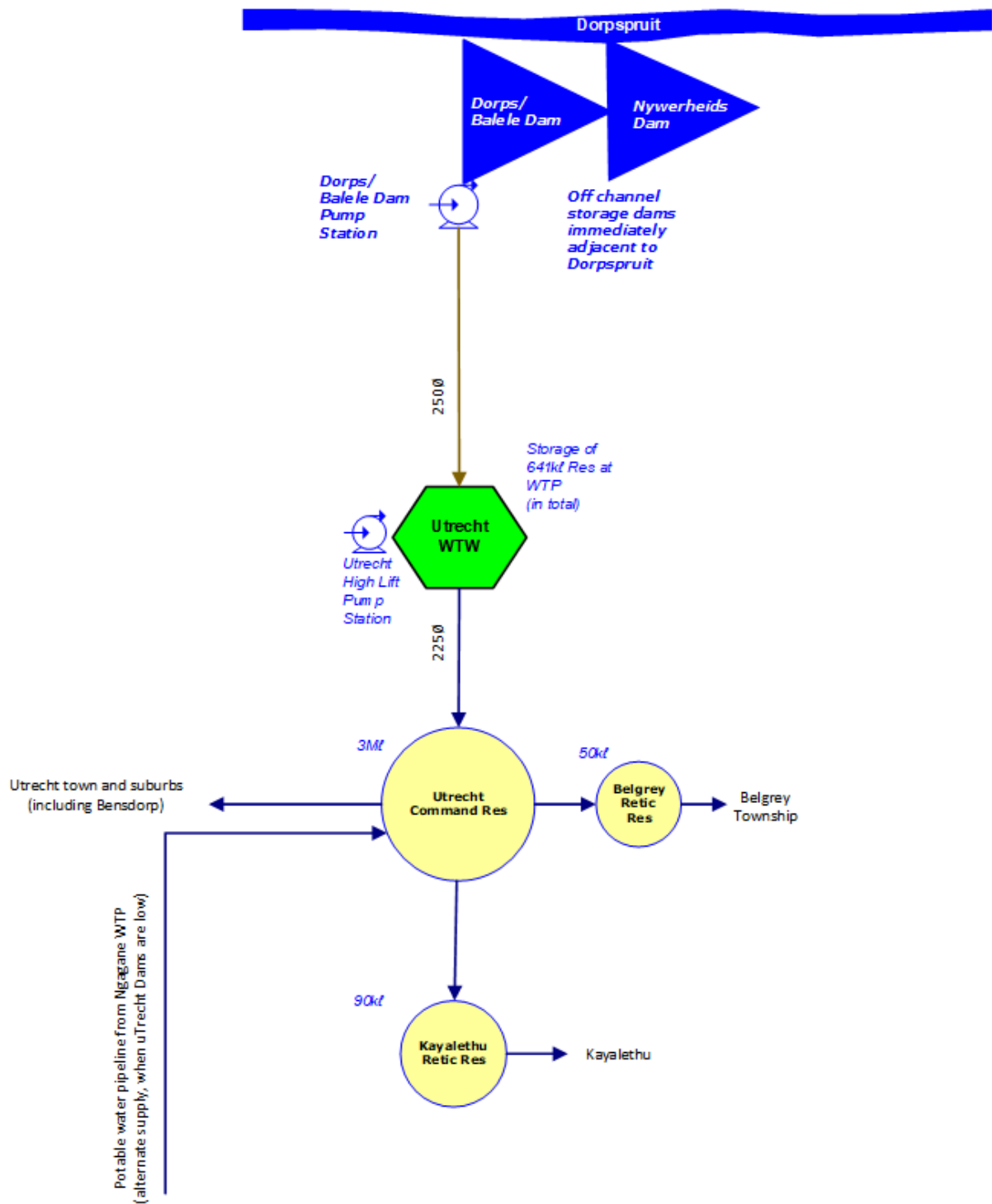
Figure 14.38 Utrecht WTP Supply Schematic (not to scale; Amajuba DM Water bulk infrastructure)
