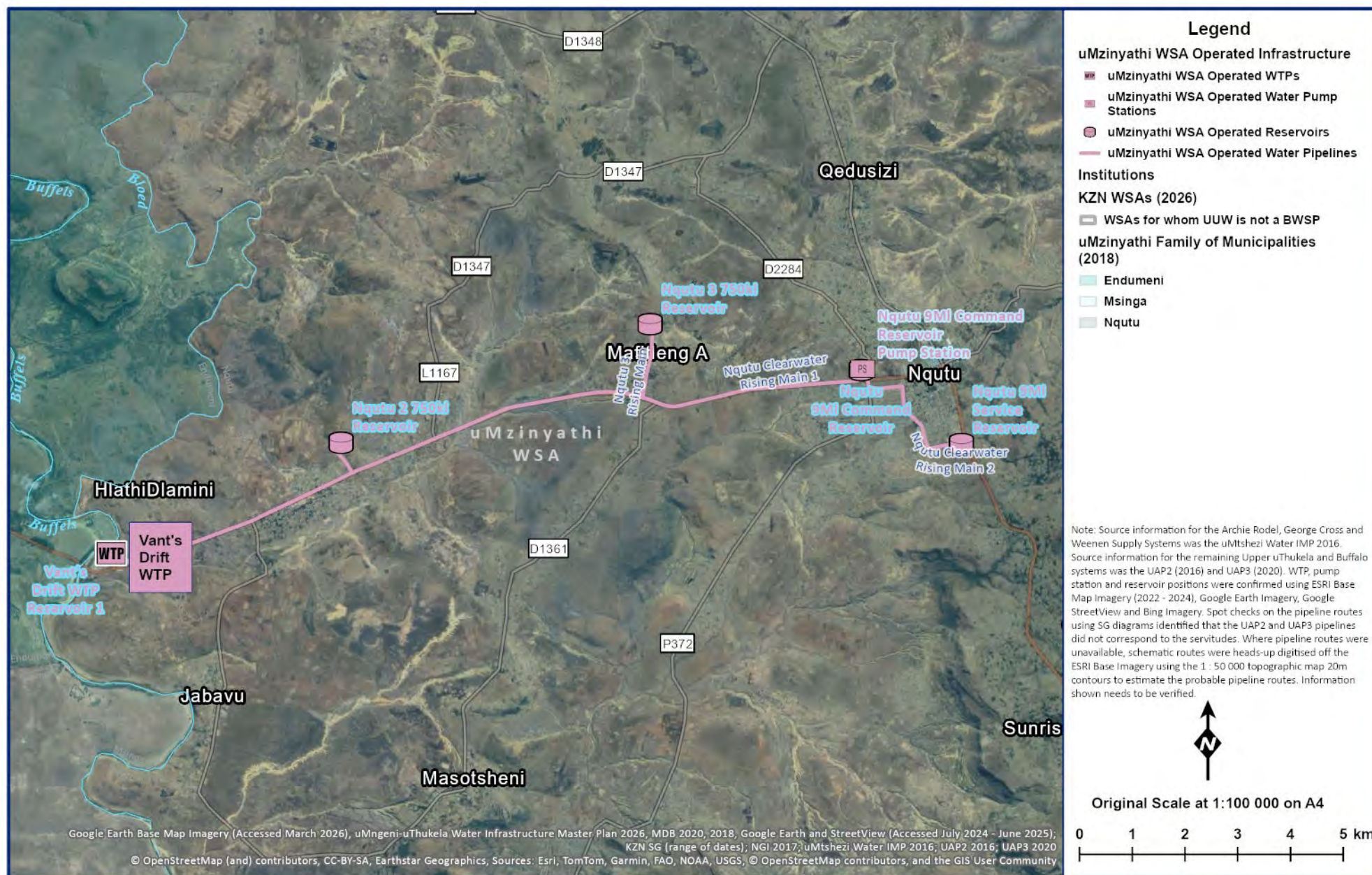
Figure 14.52 Nqutu Supply System Layout (Vants Drift WTP System).
