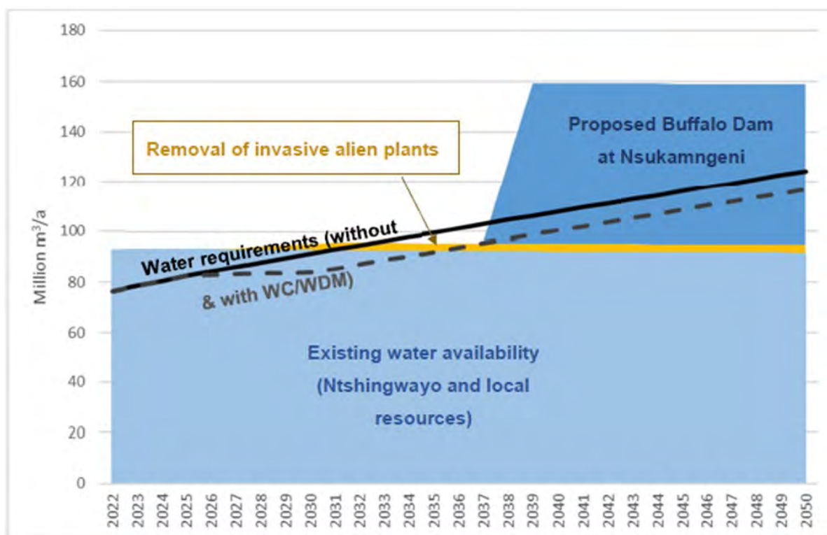
Figure 14.60 Water Balance projections for the Ngagane and Buffalo systems (DWS 2024).
