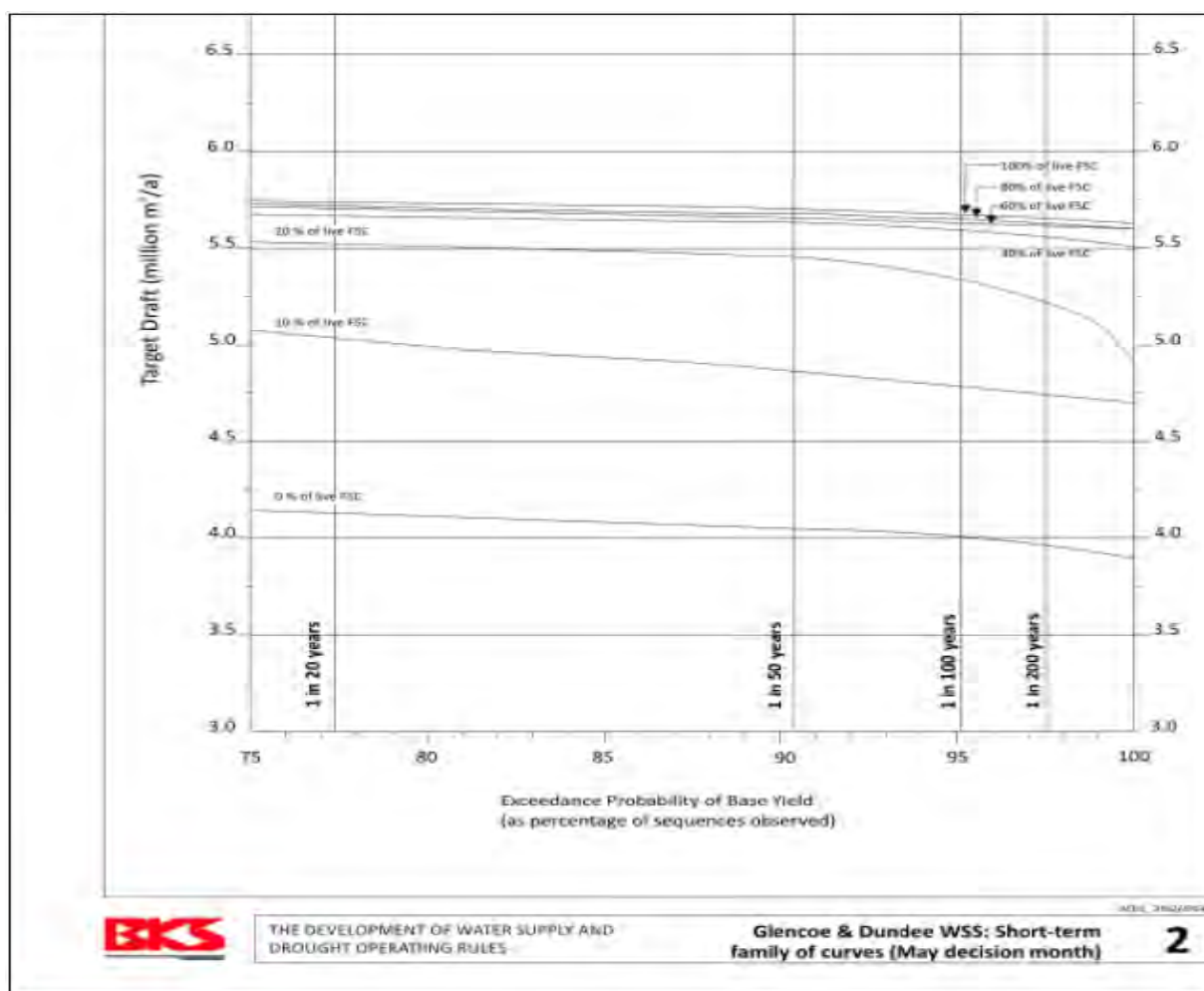
Figure 14.20 Family of curves for May decision month for the Glencoe and Dundee dams (DWS, 2022).
