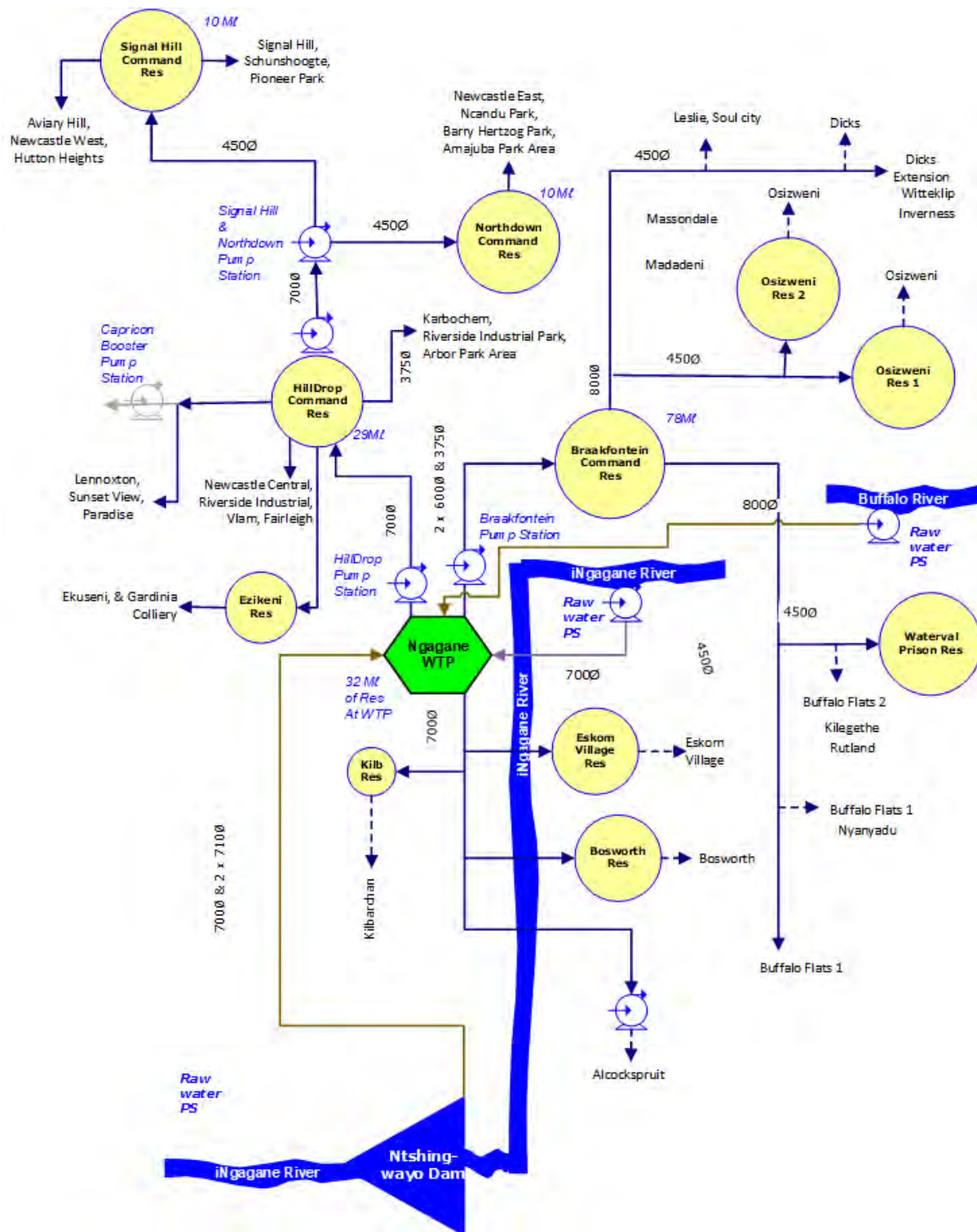
Figure 14.22 Ngagane WTP Supply System Schematic (not to scale; uThukela Water bulk infrastructure)
