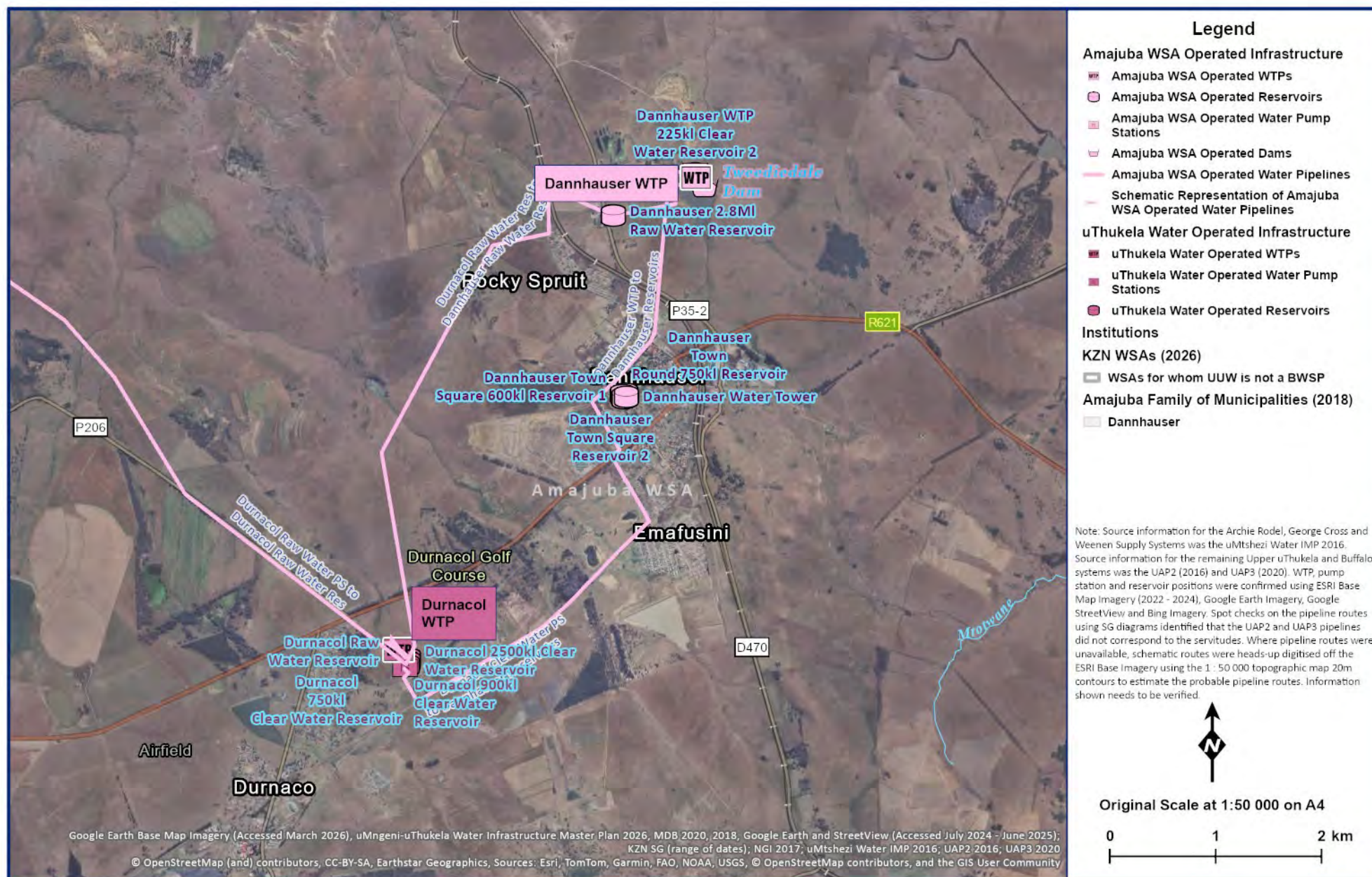
Figure 14.31 Durnacol-Dannhauser Sub-System.
