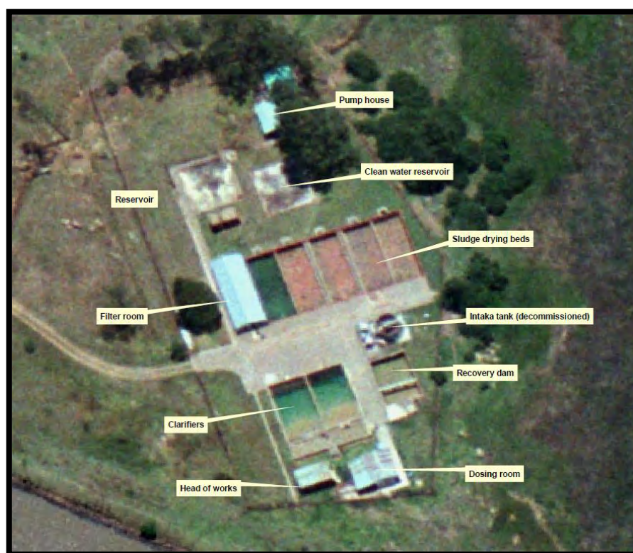
Figure 14.33 Aerial Image of Dannhauser Water Treatment Plant (ADM O&M Manual May 2016)
