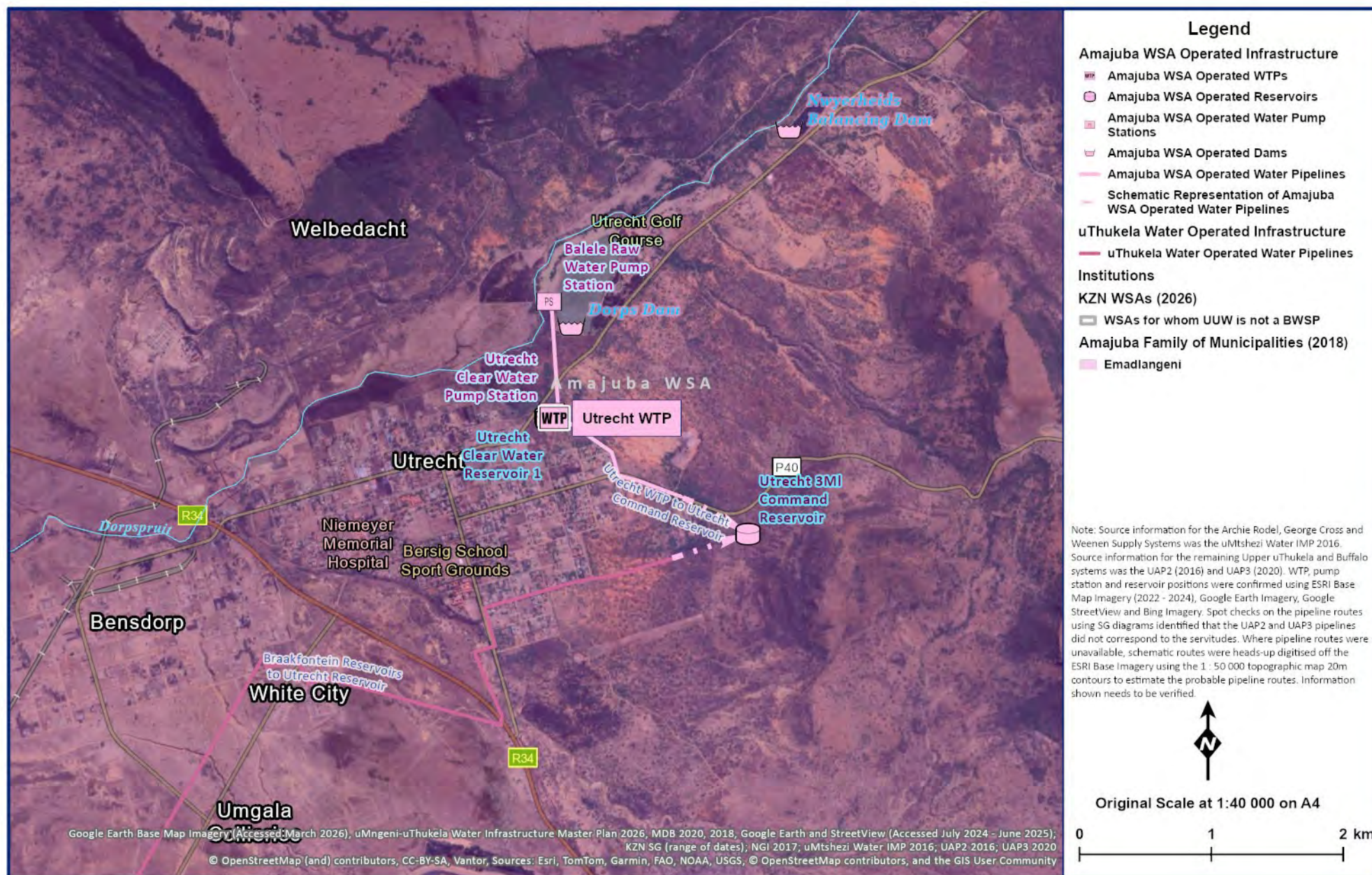
Figure 14.39 Utrecht Supply System Layout (Utrecht WTP System).
