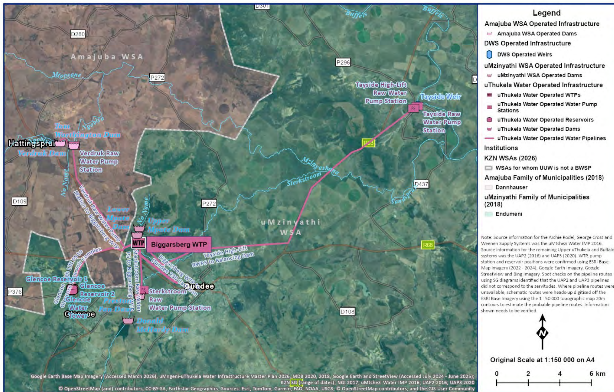
Figure 14.48 Dundee/Glencoe Supply System Layout (Biggarsberg WTP System).
