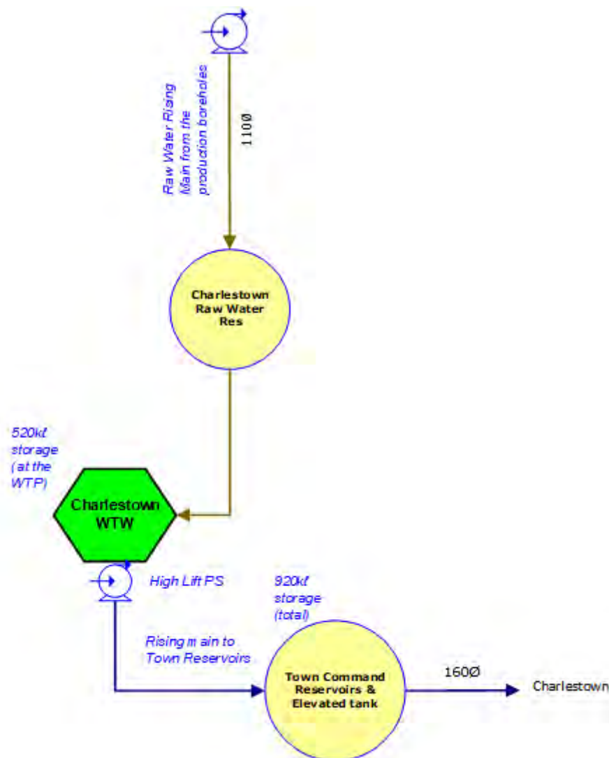
Figure 14.43 Charlestown WTP Supply Schematic (not to scale; Newcastle LM bulk water infrastructure)
