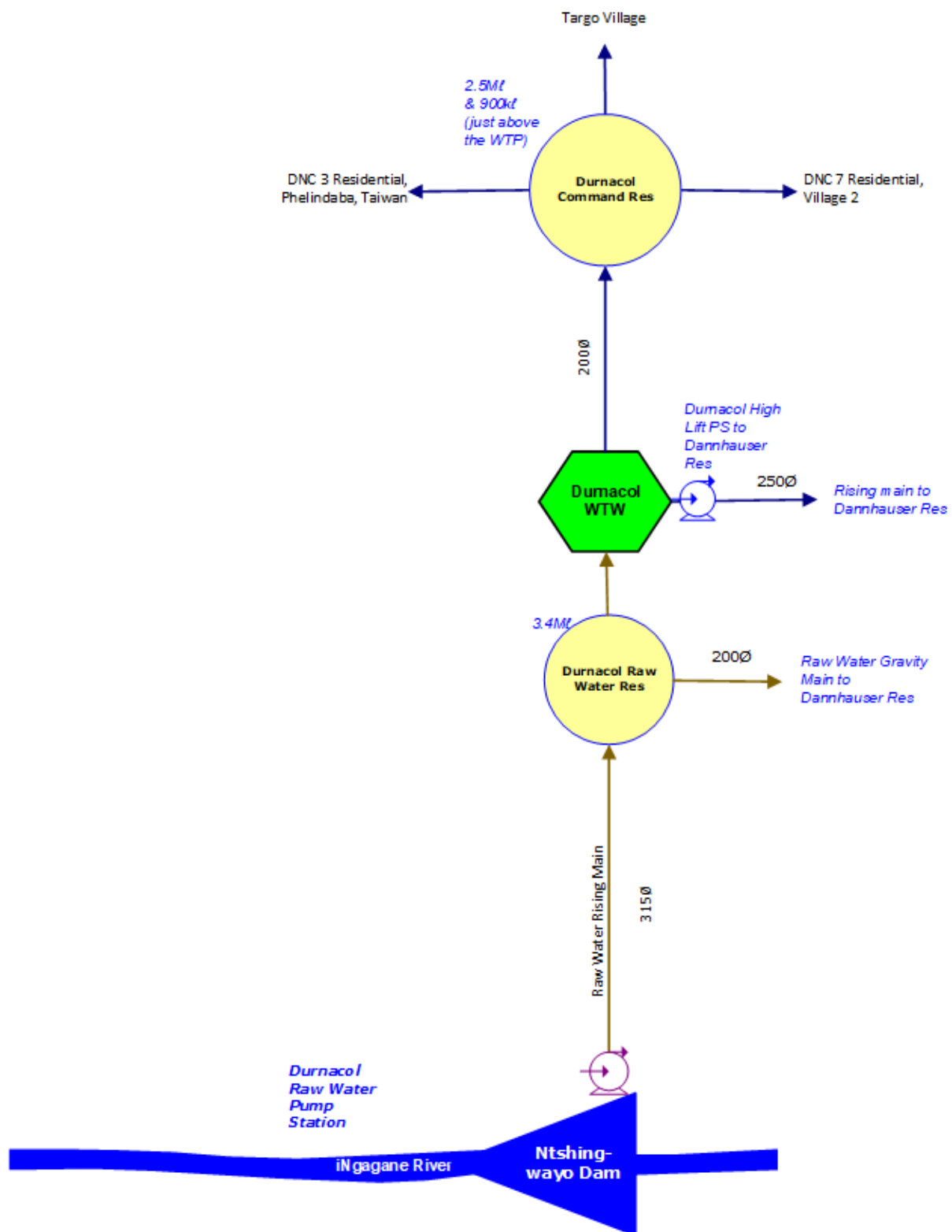
Figure 14.29 Durnacol WTP Supply Schematic (not to scale; Amajuba DM Water bulk infrastructure)
