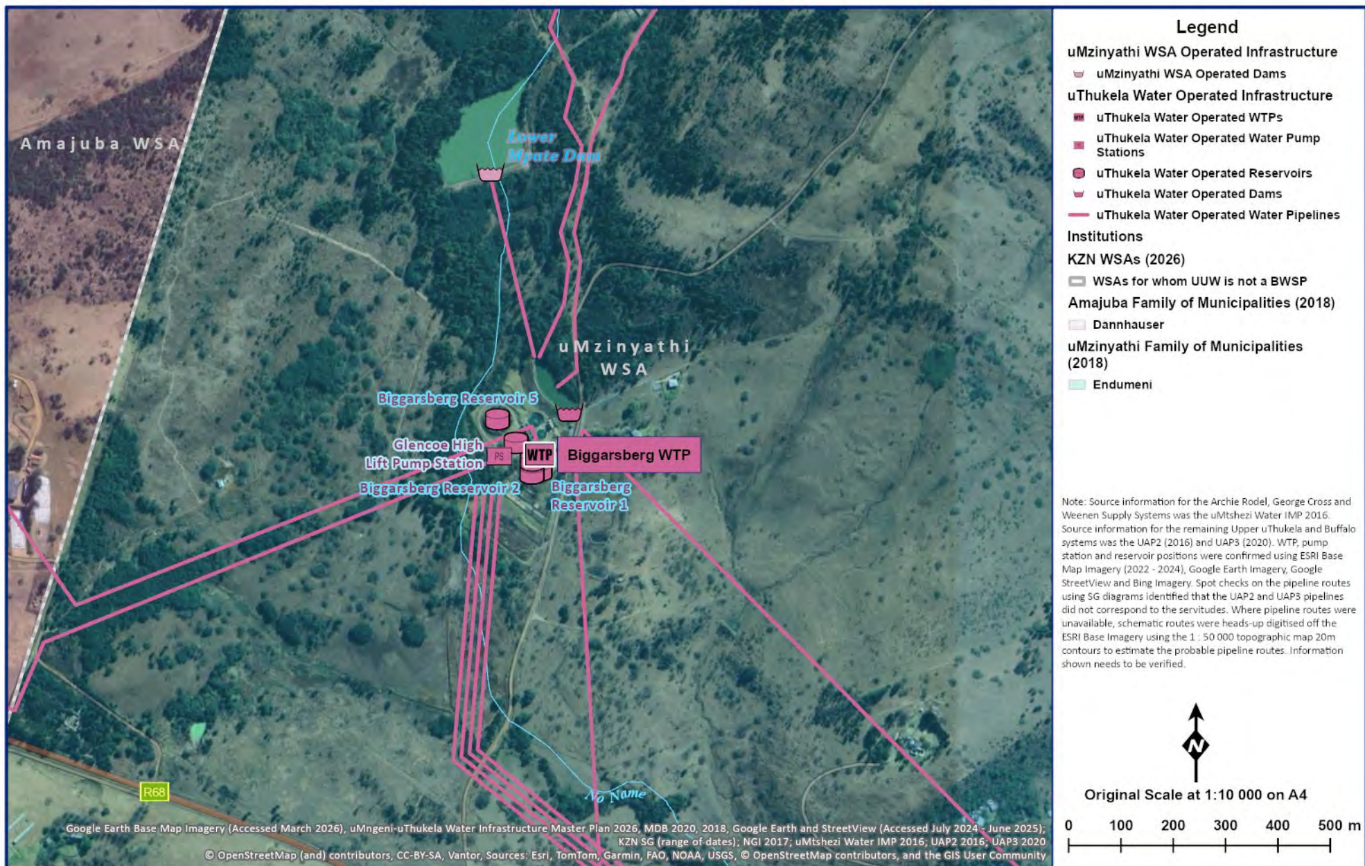
Figure 14.49 Biggarsberg WTP.
