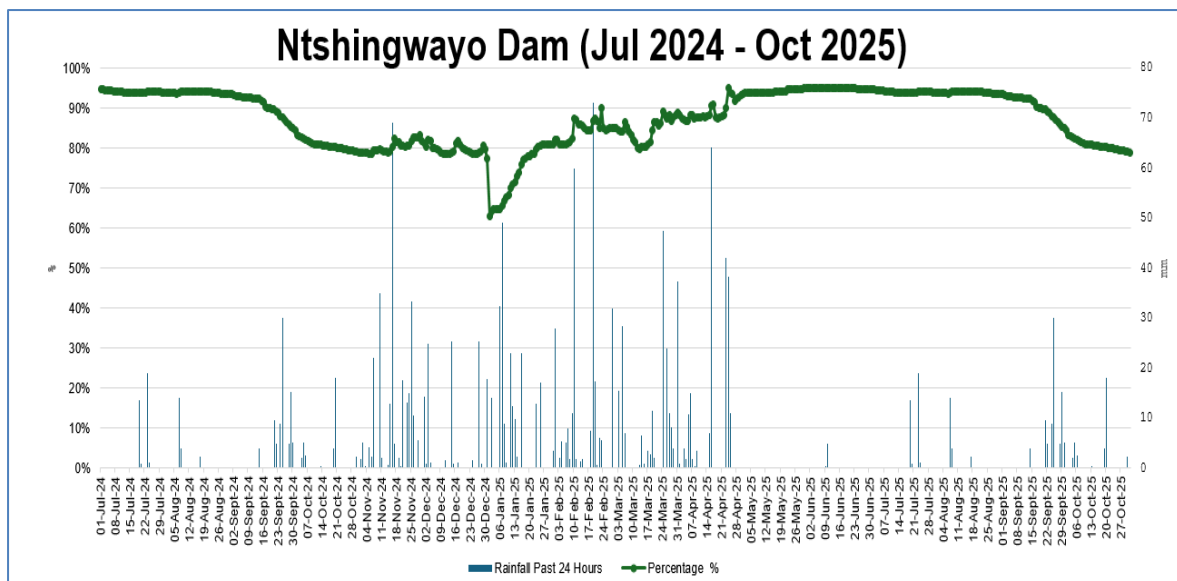
Figure 14.10 Ntshingwayo Dam level (Jul 2024 – Oct 2025).
