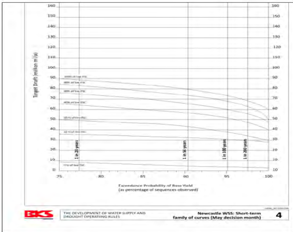
Figure 14.19 Family of curves for May decision month for the Newcastle WSS (DWS, 2022).
