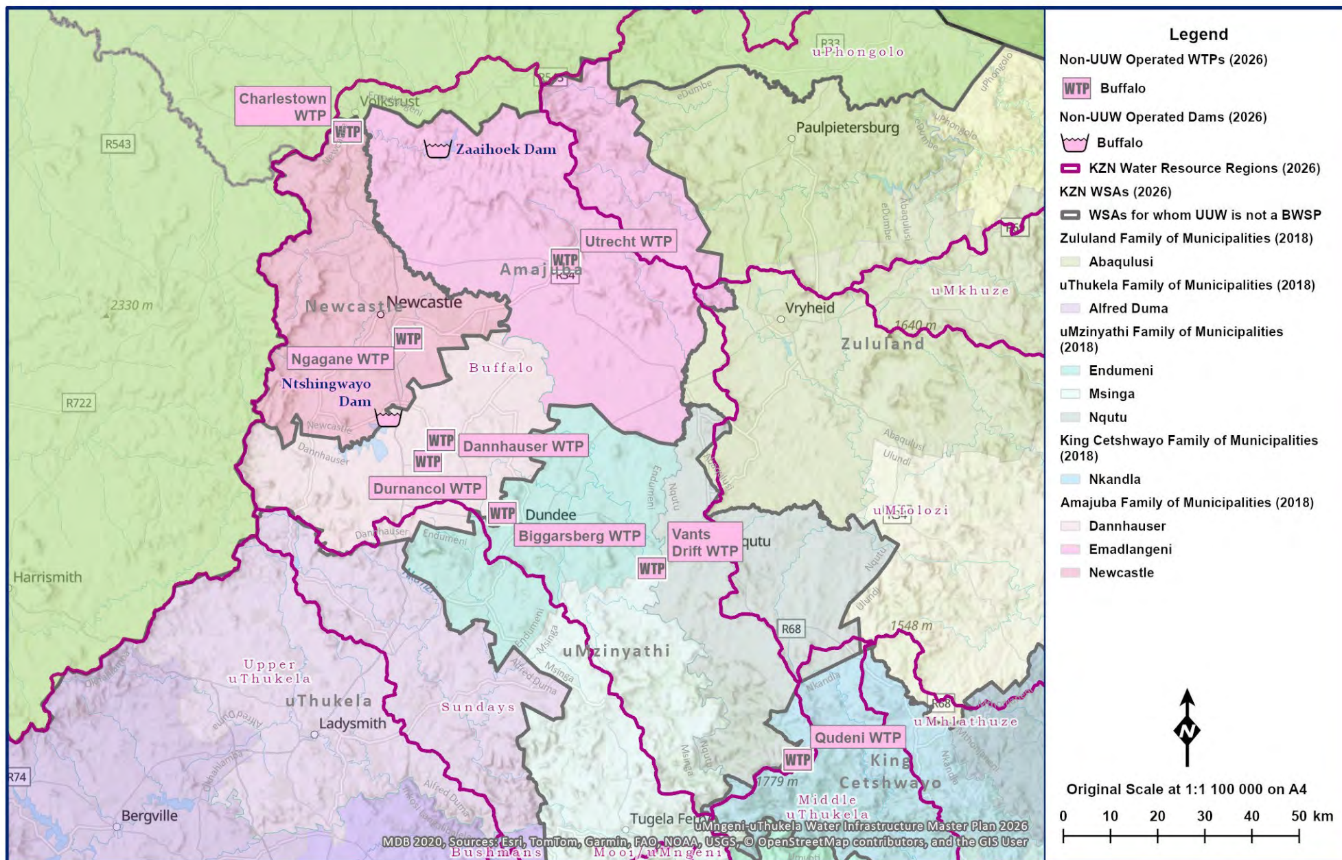
Figure 14.2 General Layout of the Buffalo System.
