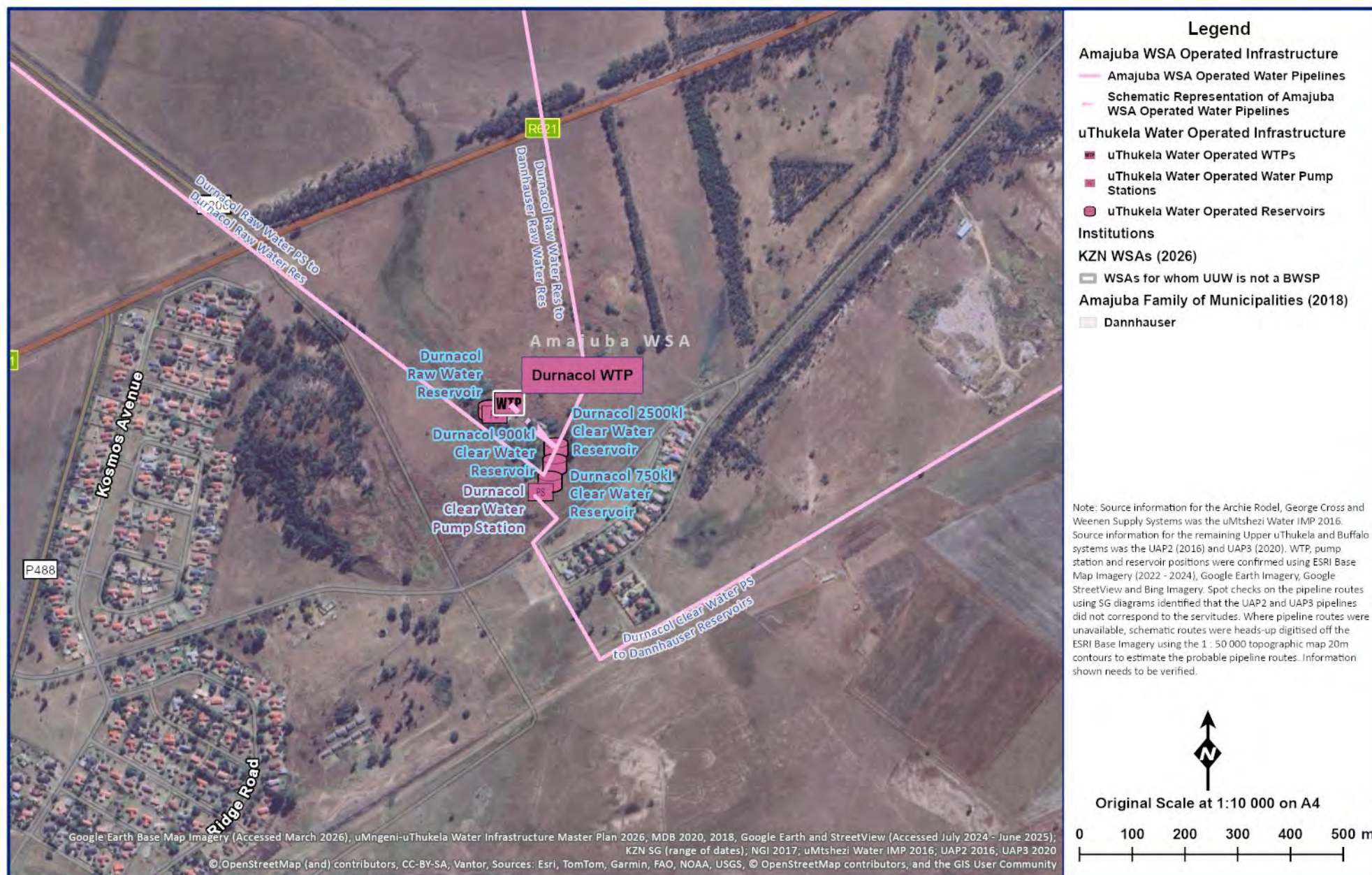
Figure 14.30 Durnacol Supply System Layout (Durnacol WTP System).
