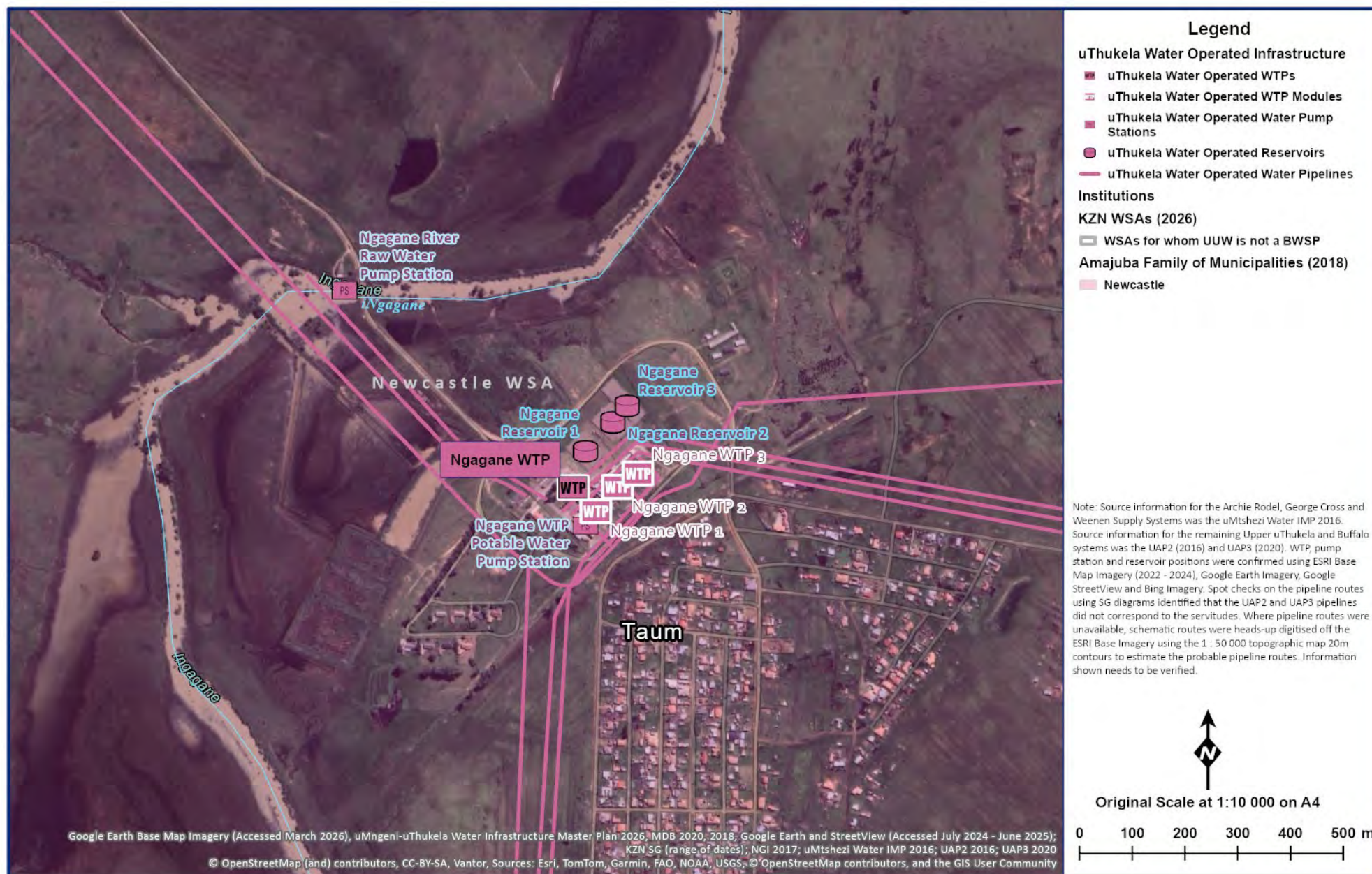
Figure 14.24 Ngagane WTP.
