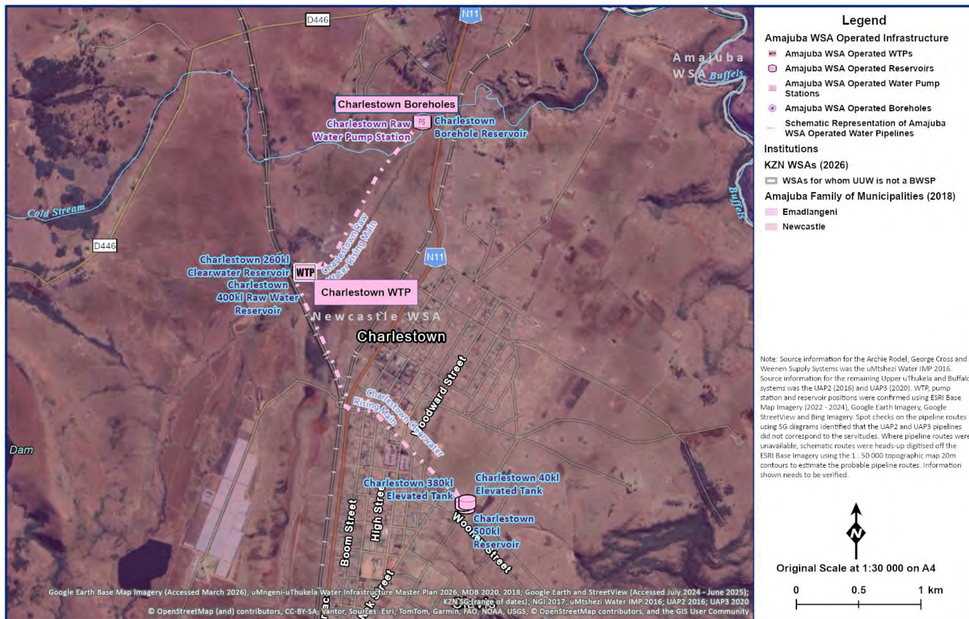
Figure 14.44 Charlestown Supply System Layout (Charlestown WTP System).
