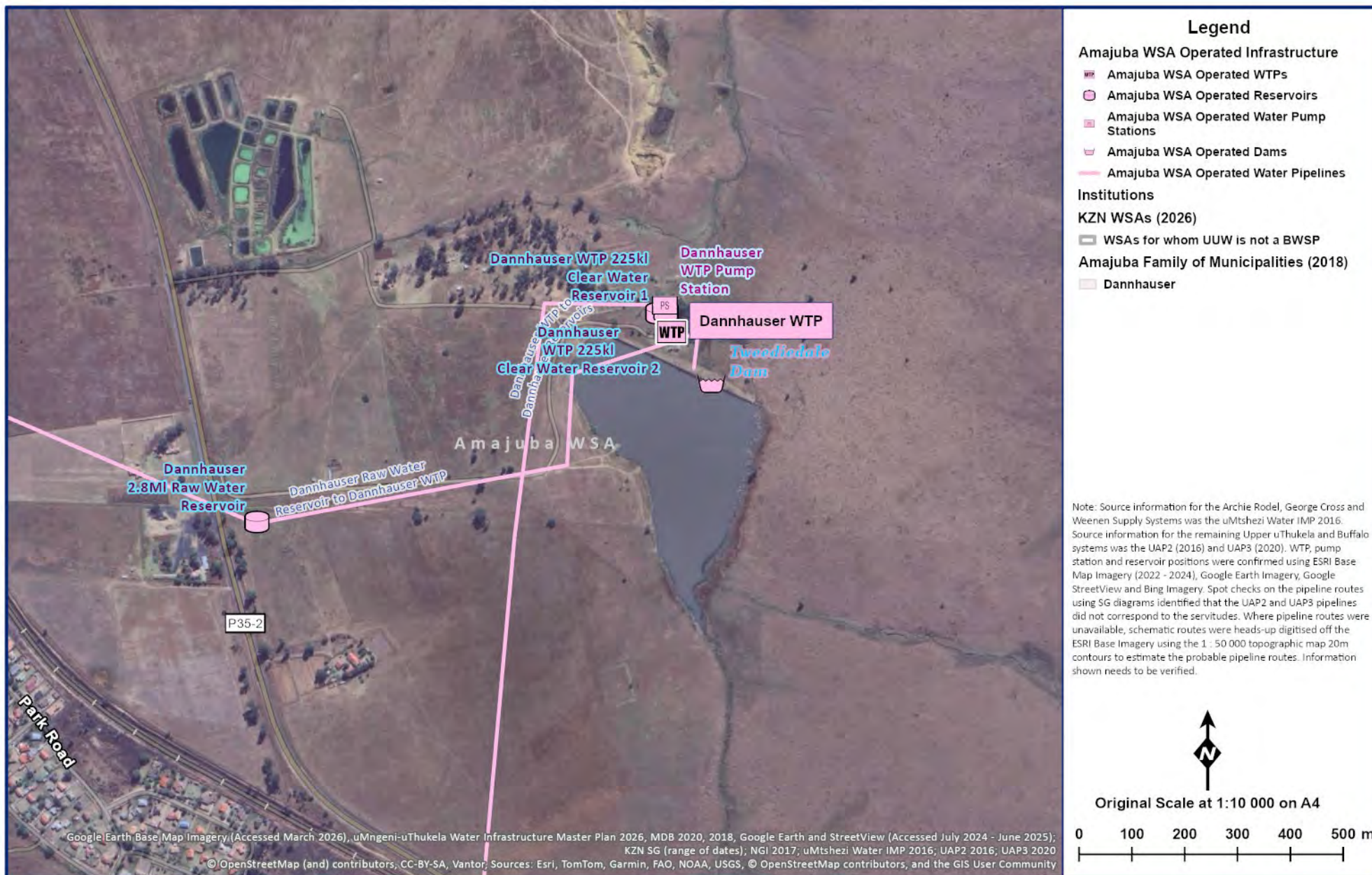
Figure 14.35 Dannhauser Supply System Layout.
