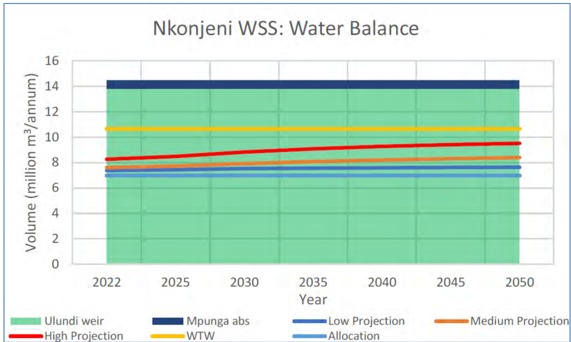
Figure 17.31 Nkonjeni RBWSS water balance
