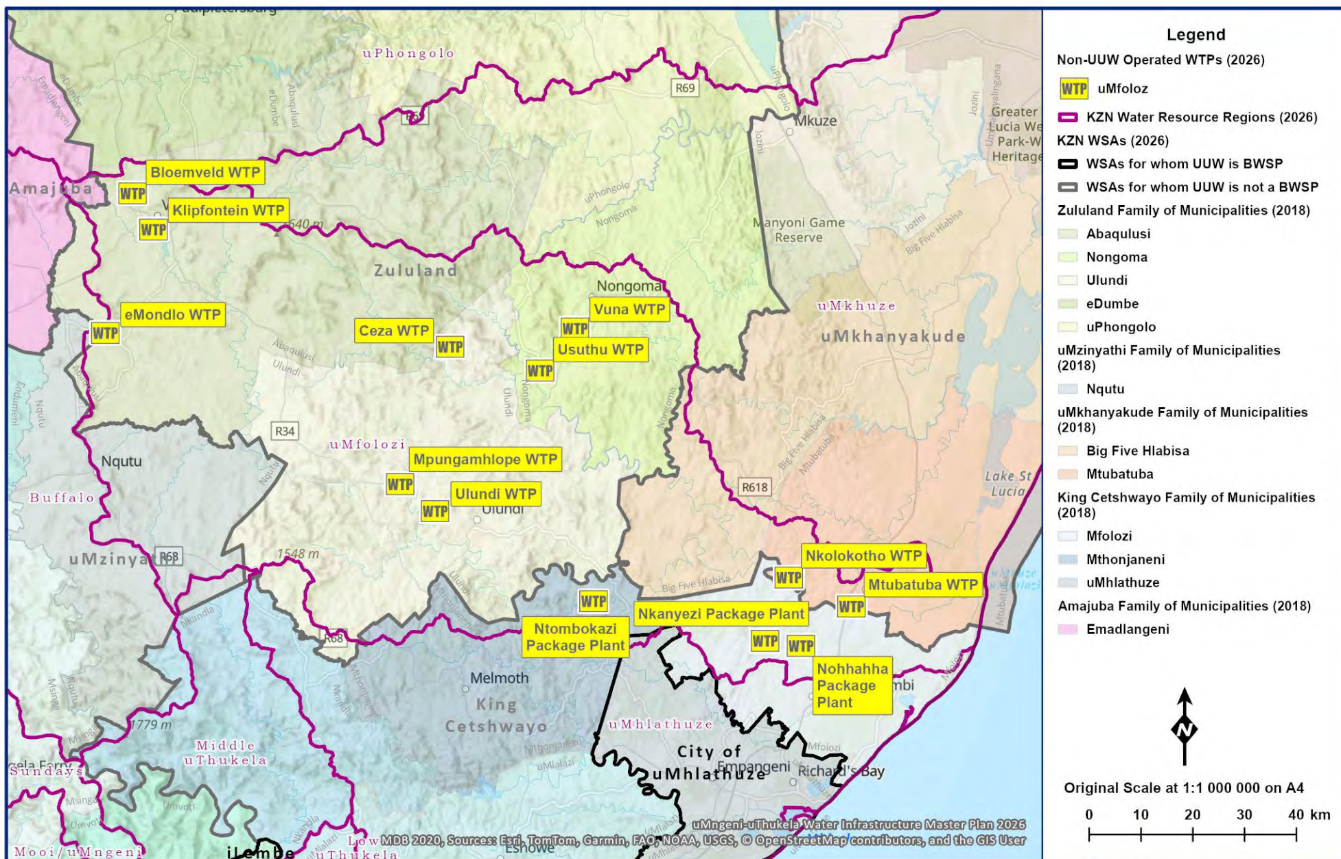
Figure 17.1 General layout of the uMfolozi System.
