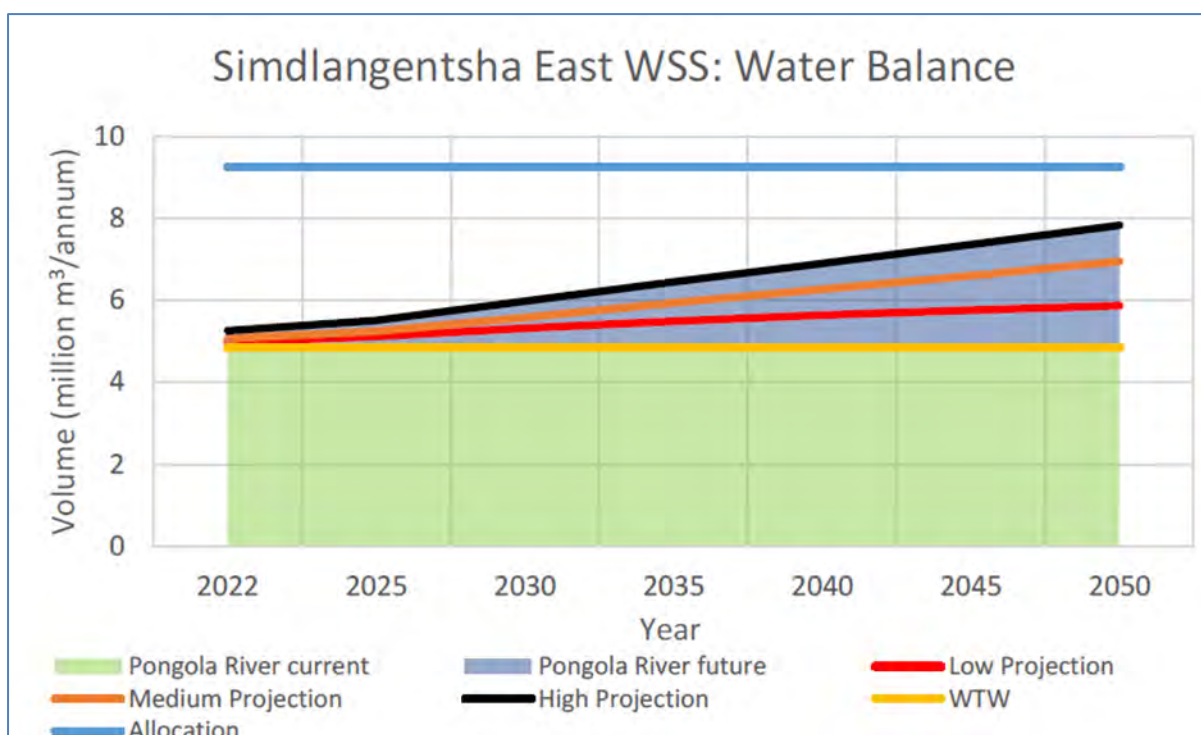
Figure 18.43 Simdlangentsha East WSS water balance
