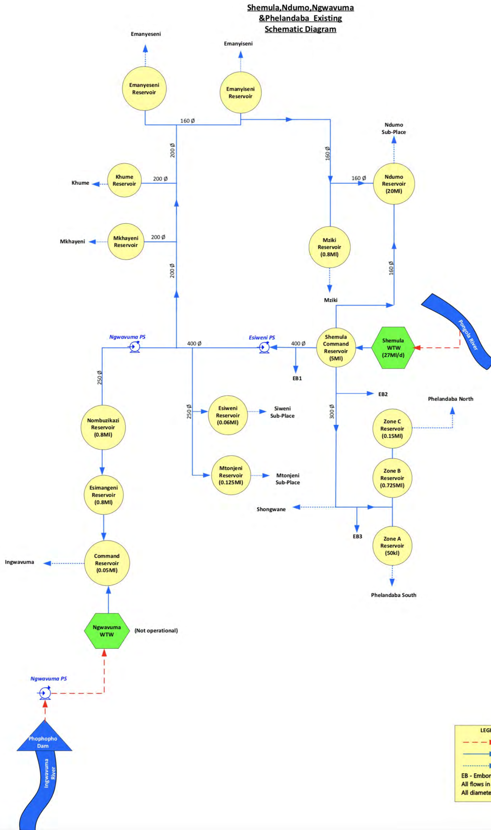
Figure 18.37 Schematic showing the Shemula Supply System
