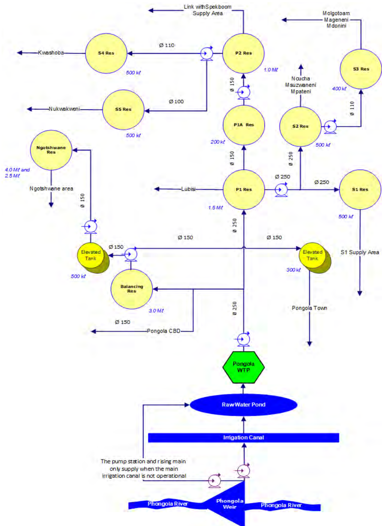
Figure 18.27 Schematic of Phongola WTP Supply System
