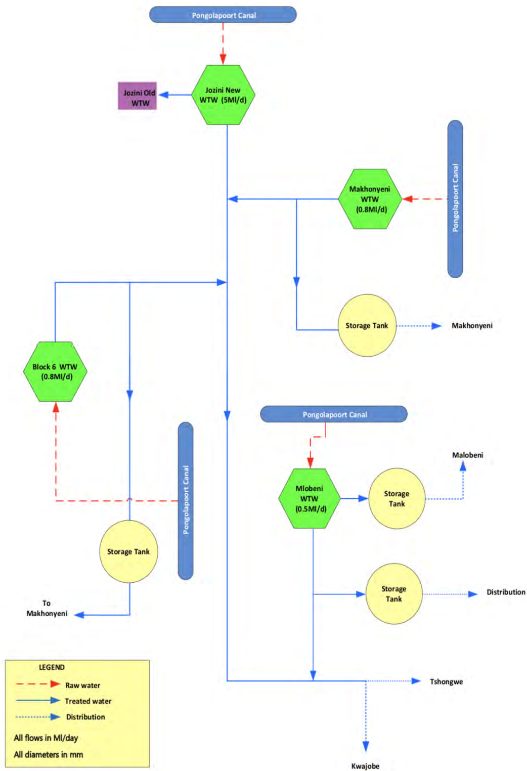
Figure 18.32 Schematic of Jozini WTP Supply System
