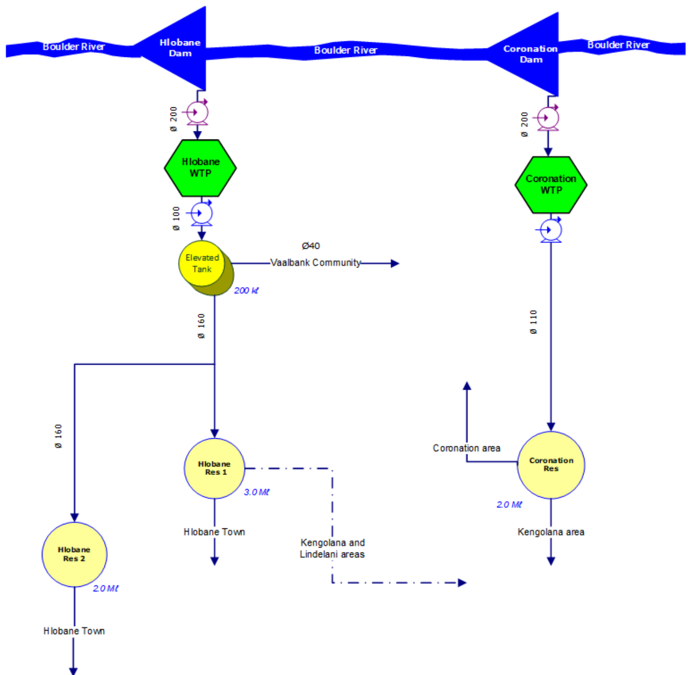
Figure 18.20 Schematic of the Hlobane/Coronation Supply System.
