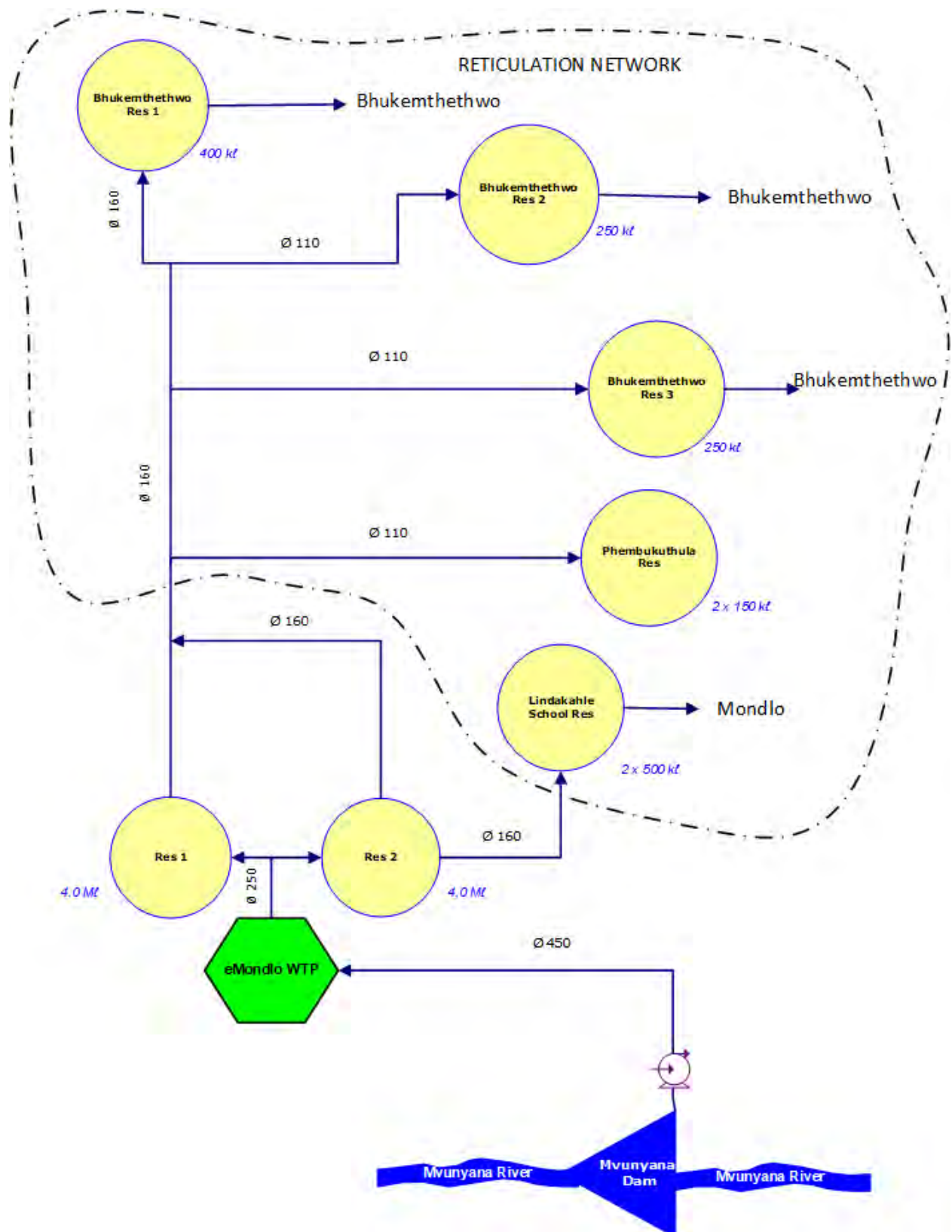
Figure 17.29 Schematic of the eMondlo Supply System
