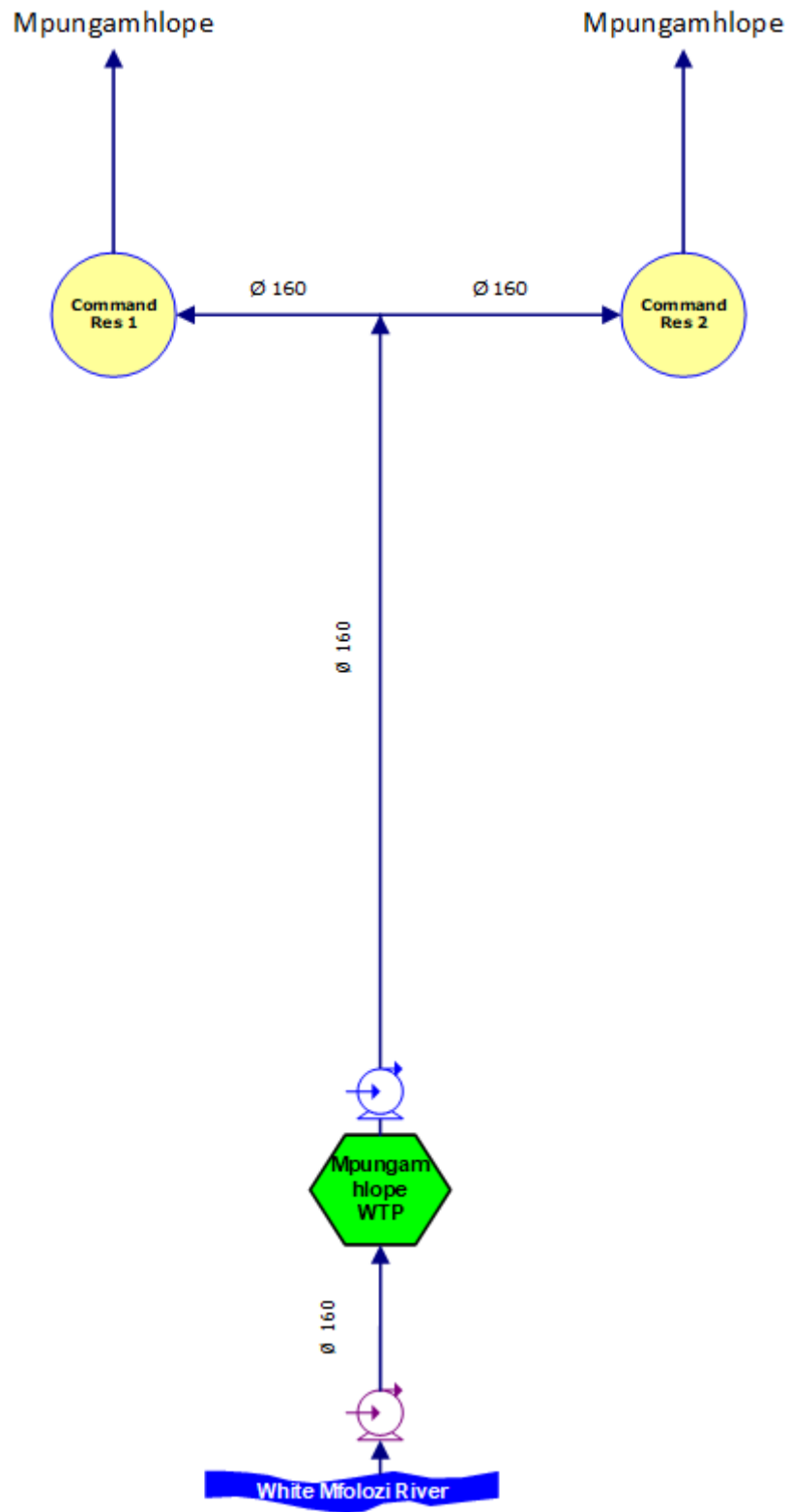
Figure 17.19 Schematic of the Mpungamhlope Supply System
