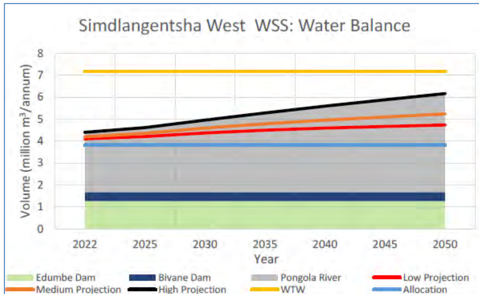
Figure 18.44 Simdlangentsha West WSS water balance
