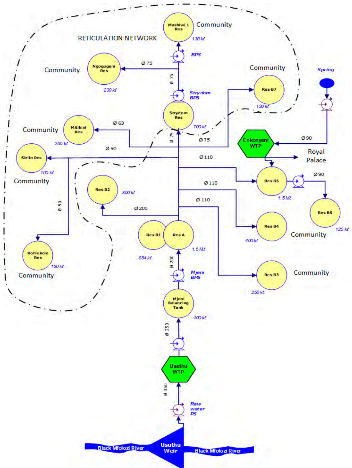
Figure 17.21 Schematic of the Usuthu Supply System
