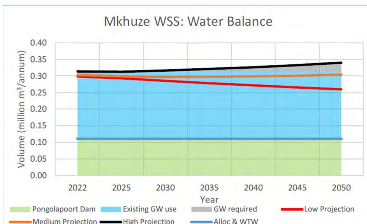
Figure 18.40 Mkhuzi WSS water balance
