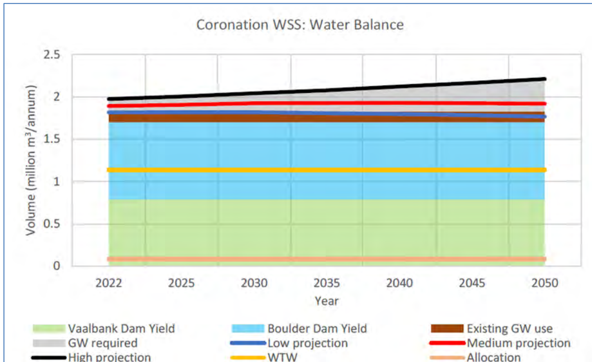
Figure 18.41 Coronation WSS water balance
