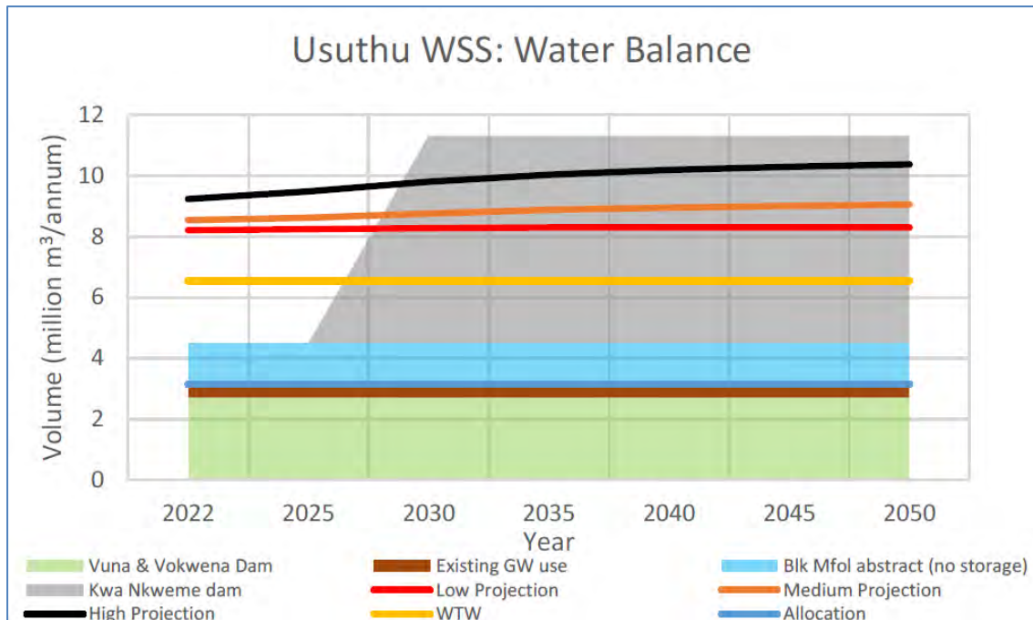
Figure 17.32 Usuthu RBWSS water balance
