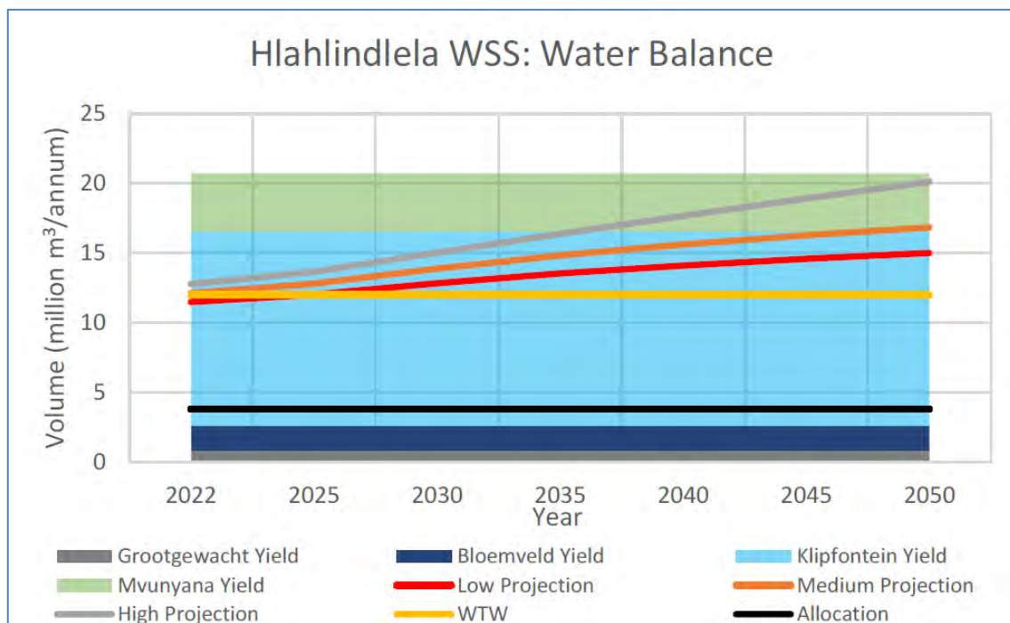
Figure 17.30 Hlahlindlela WSS water balance
